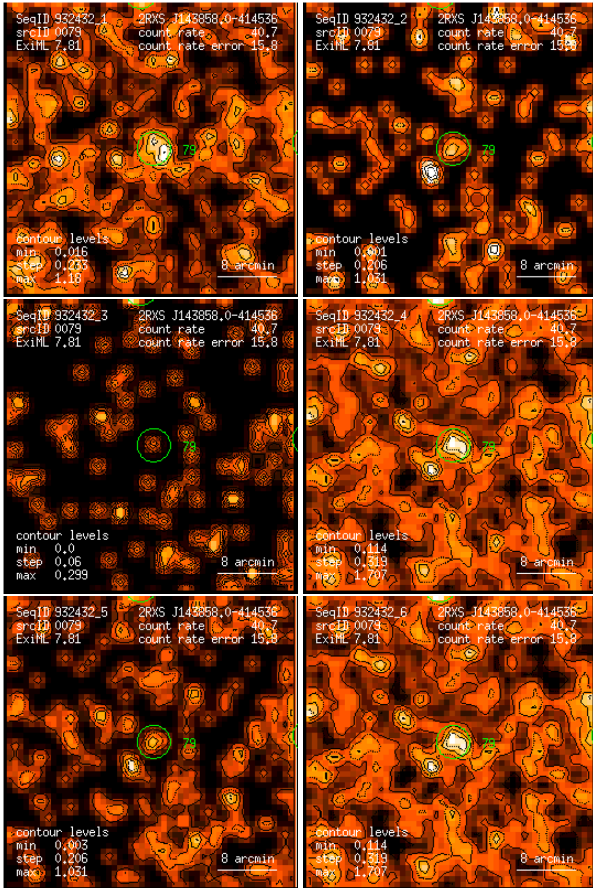
Figure 79: RASS 932432: detection 0079: band rate images, Gaussian filter: (1) PSPC channels 11 – 41, (2) 52 – 90, (3) 91 – 201, (4) 11 – 235, (5) 52 – 201, (6) 11 – 201. Broad band rates in counts/ks. Band rate contour levels in counts/ks/arcmin 2 .
