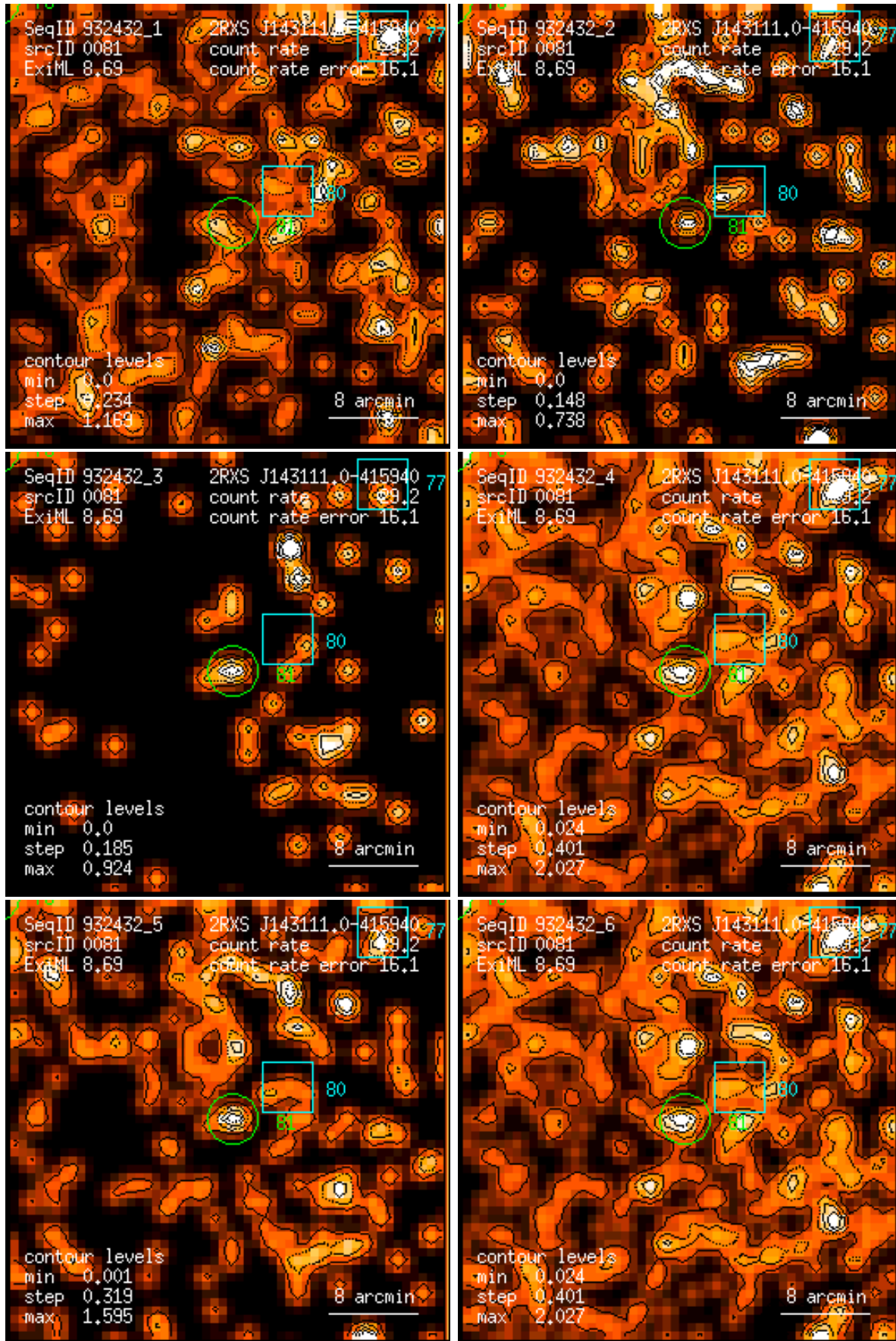
Figure 81: RASS 932432: detection 0081: band rate images, Gaussian filter: (1) PSPC channels 11 – 41, (2) 52 – 90, (3) 91 – 201, (4) 11 – 235, (5) 52 – 201, (6) 11 – 201. Broad band rates in counts/ks. Band rate contour levels in counts/ks/arcmin 2 .
