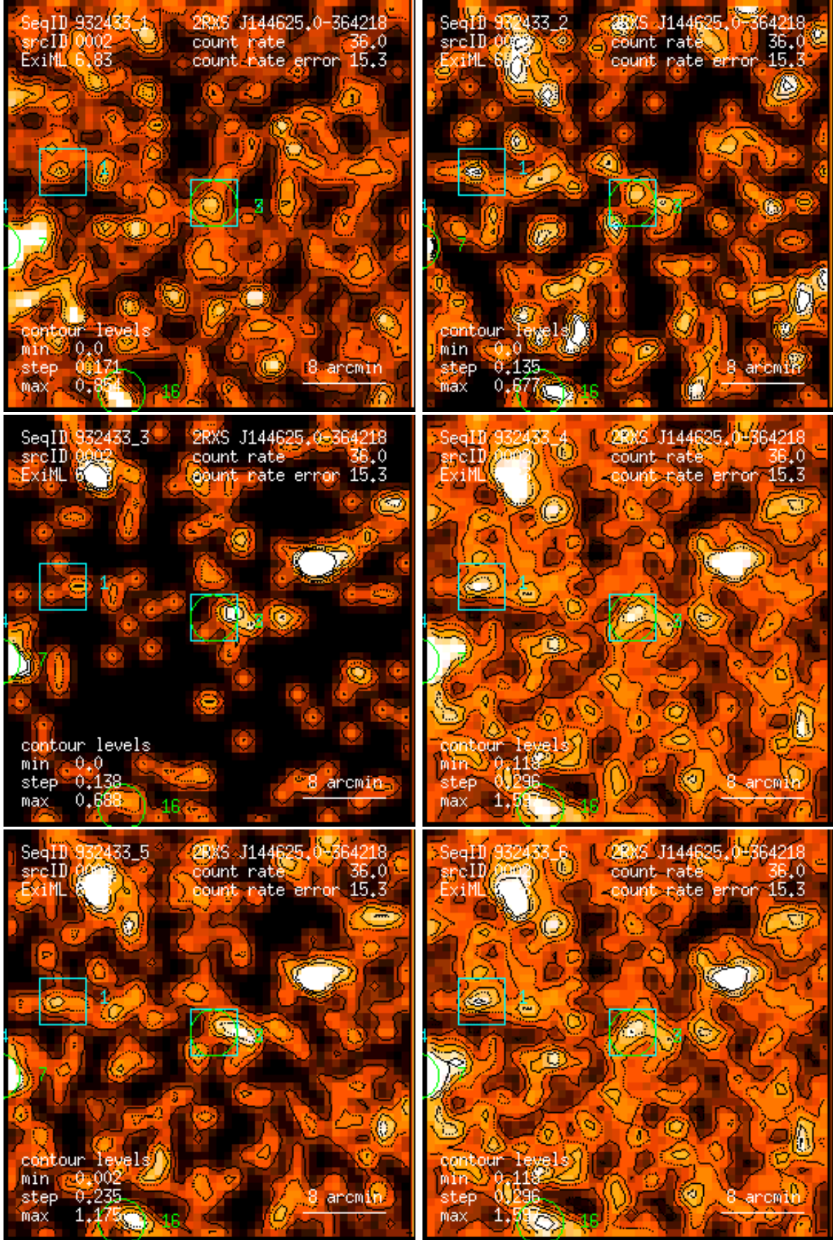
Figure 2: RASS 932433: detection 0002: band rate images, Gaussian filter: (1) PSPC channels 11 – 41, (2) 52 – 90, (3) 91 – 201, (4) 11 – 235, (5) 52 – 201, (6) 11 – 201. Broad band rates in counts/ks. Band rate contour levels in counts/ks/arcmin 2 .
