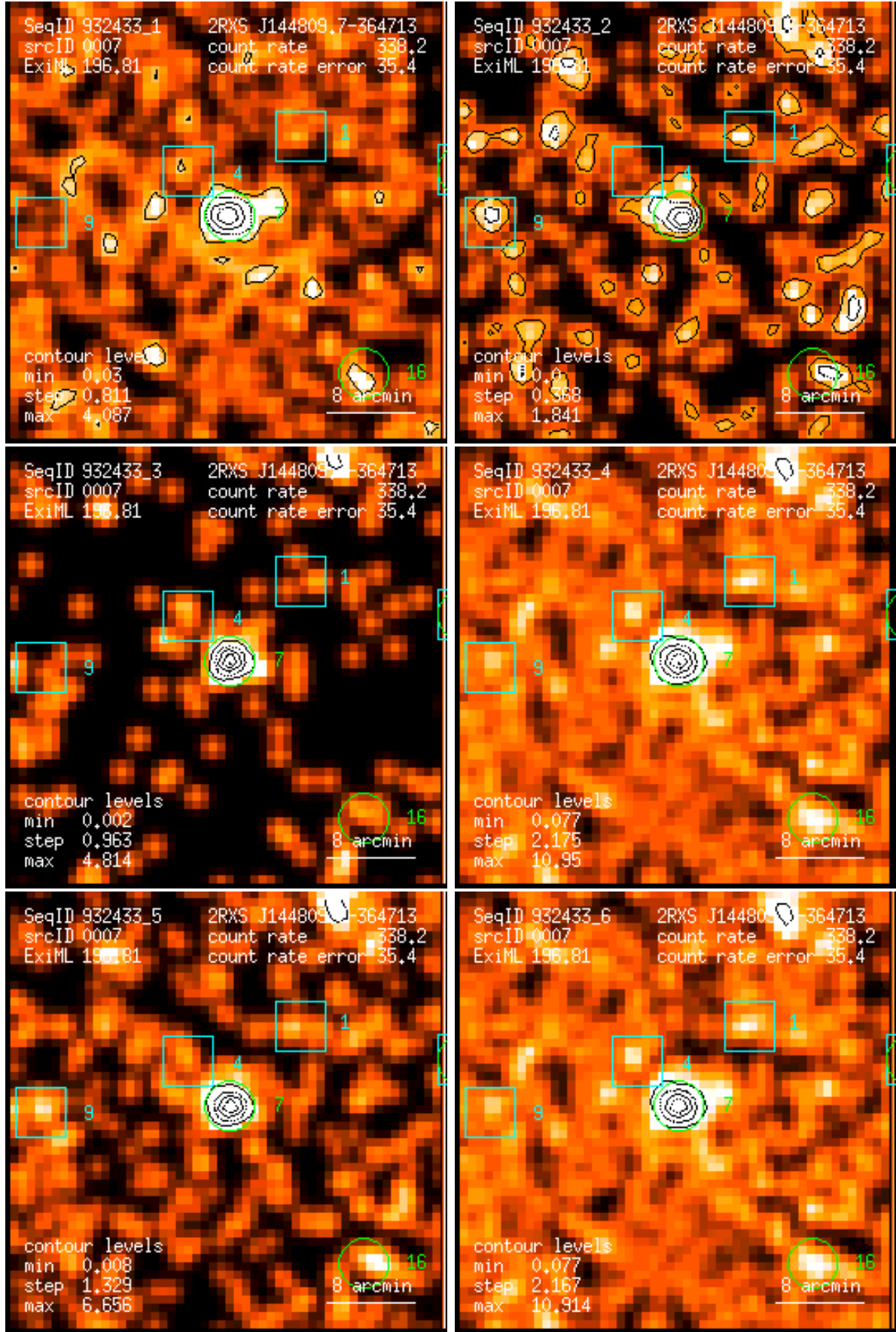
Figure 7: RASS 932433: detection 0007: band rate images, Gaussian filter: (1) PSPC channels 11 – 41, (2) 52 – 90, (3) 91 – 201, (4) 11 – 235, (5) 52 – 201, (6) 11 – 201. Broad band rates in counts/ks. Band rate contour levels in counts/ks/arcmin 2 .
