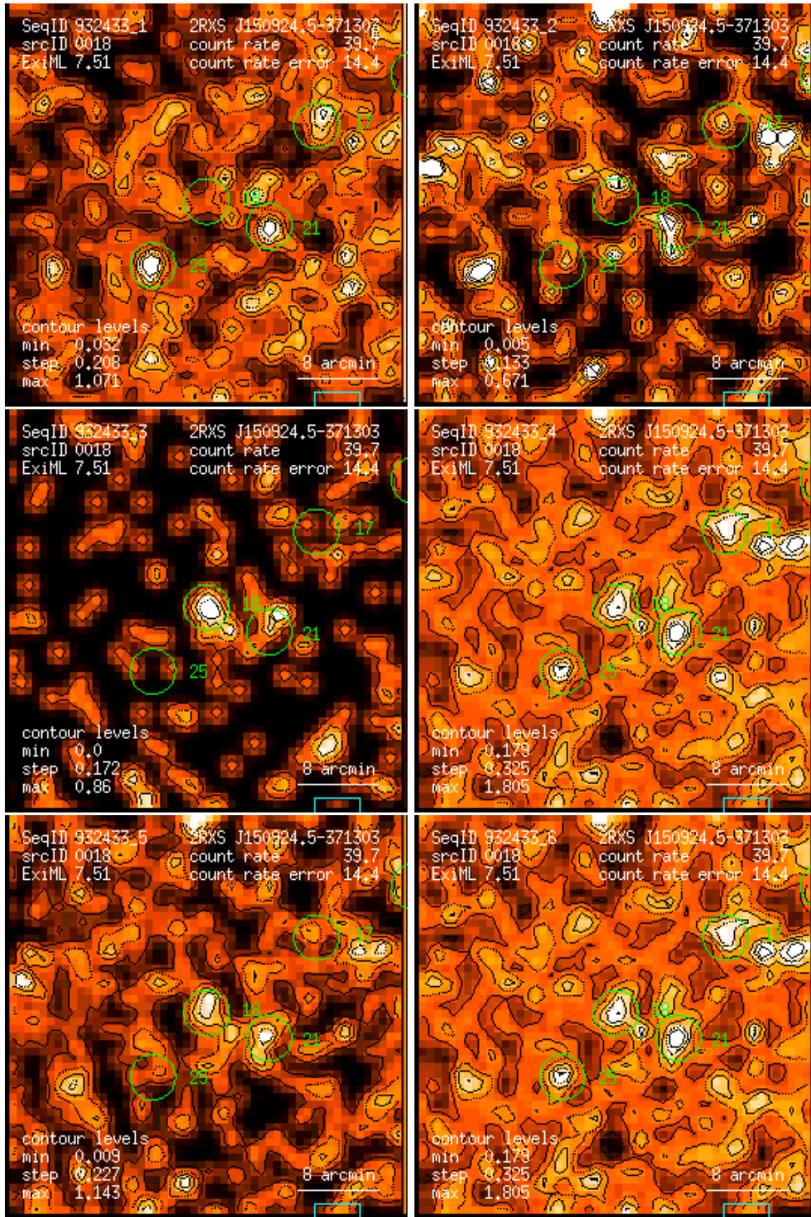
Figure 18: RASS 932433: detection 0018: band rate images, Gaussian filter: (1) PSPC channels 11 – 41, (2) 52 – 90, (3) 91 – 201, (4) 11 – 235, (5) 52 – 201, (6) 11 – 201. Broad band rates in counts/ks. Band rate contour levels in counts/ks/arcmin 2 .
