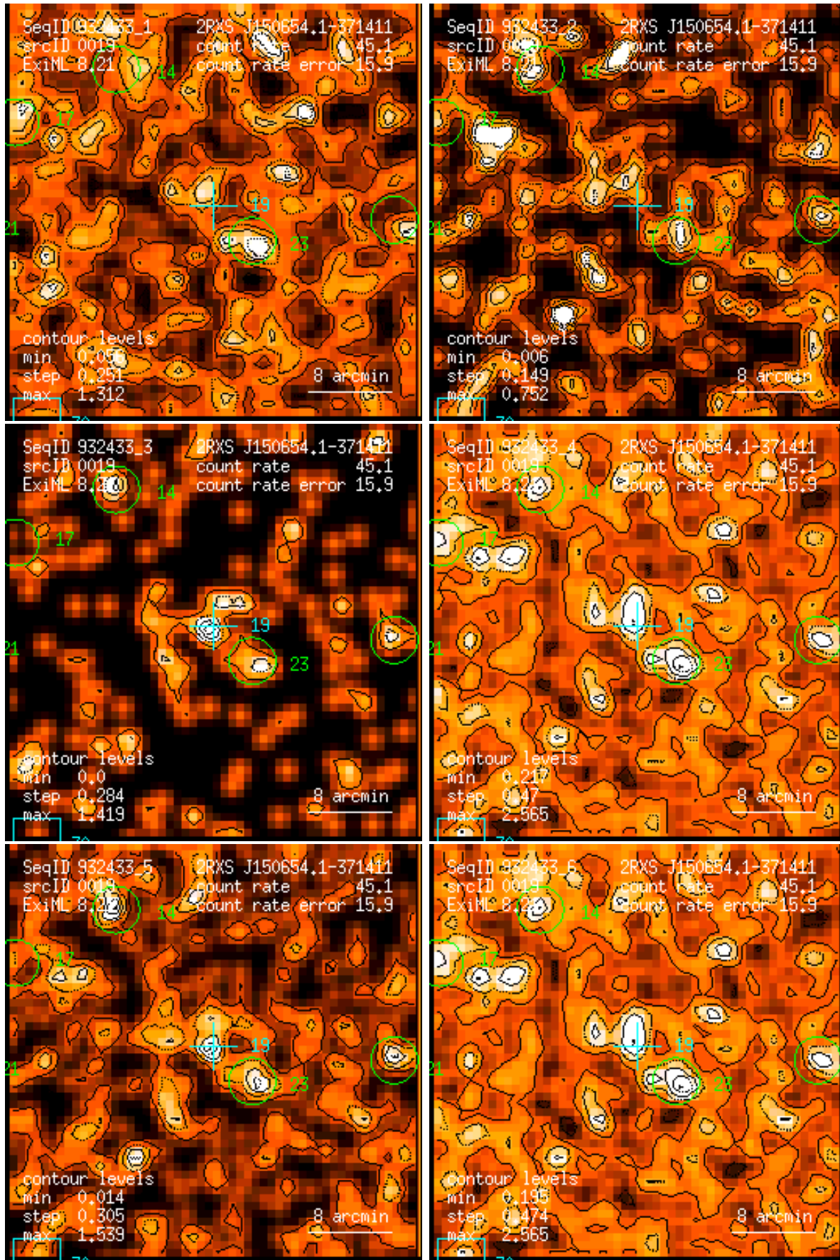
Figure 19: RASS 932433: detection 0019: band rate images, Gaussian filter: (1) PSPC channels 11 – 41, (2) 52 – 90, (3) 91 – 201, (4) 11 – 235, (5) 52 – 201, (6) 11 – 201. Broad band rates in counts/ks. Band rate contour levels in counts/ks/arcmin 2 .
