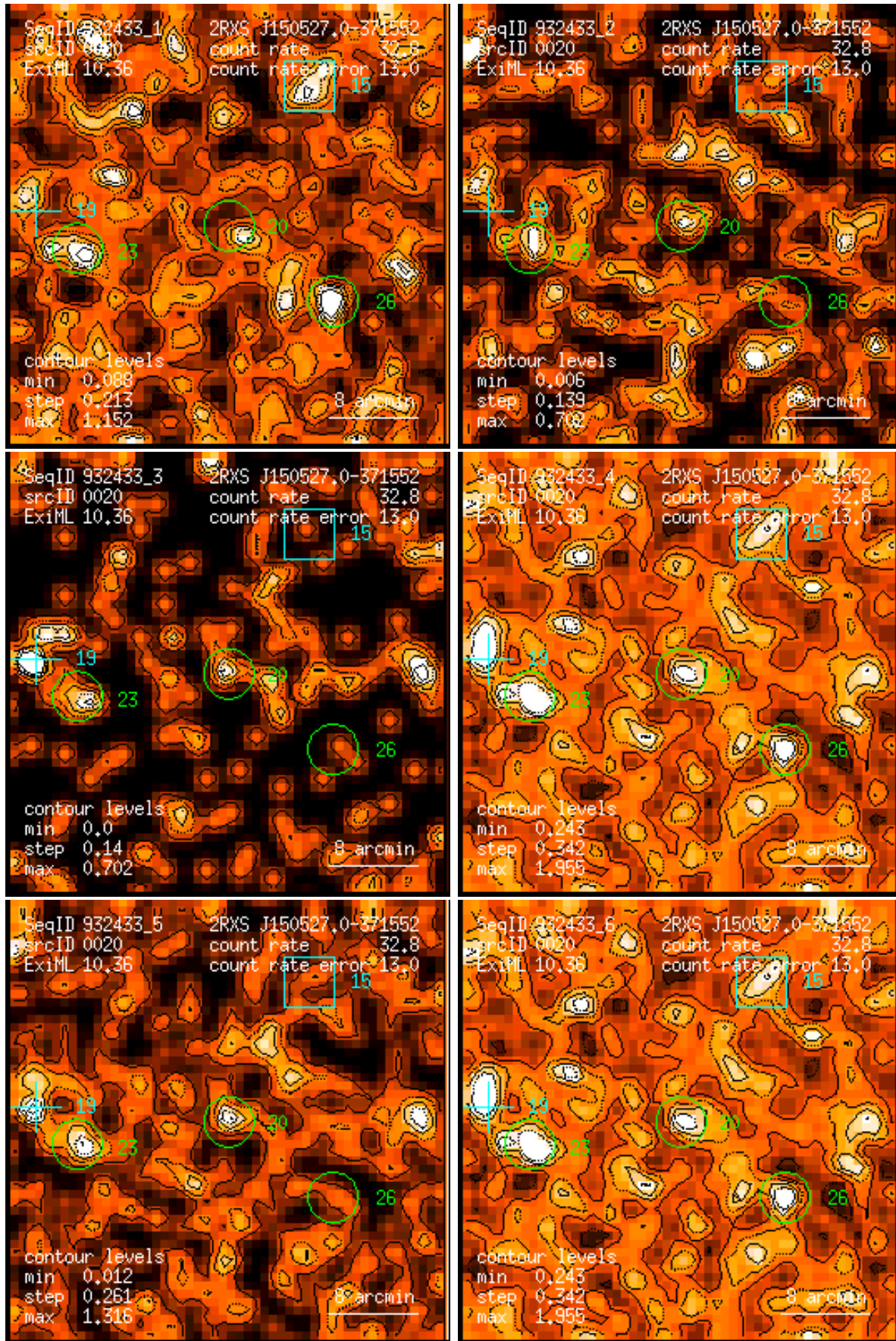
Figure 20: RASS 932433: detection 0020: band rate images, Gaussian filter: (1) PSPC channels 11 – 41, (2) 52 – 90, (3) 91 – 201, (4) 11 – 235, (5) 52 – 201, (6) 11 – 201. Broad band rates in counts/ks. Band rate contour levels in counts/ks/arcmin 2 .
