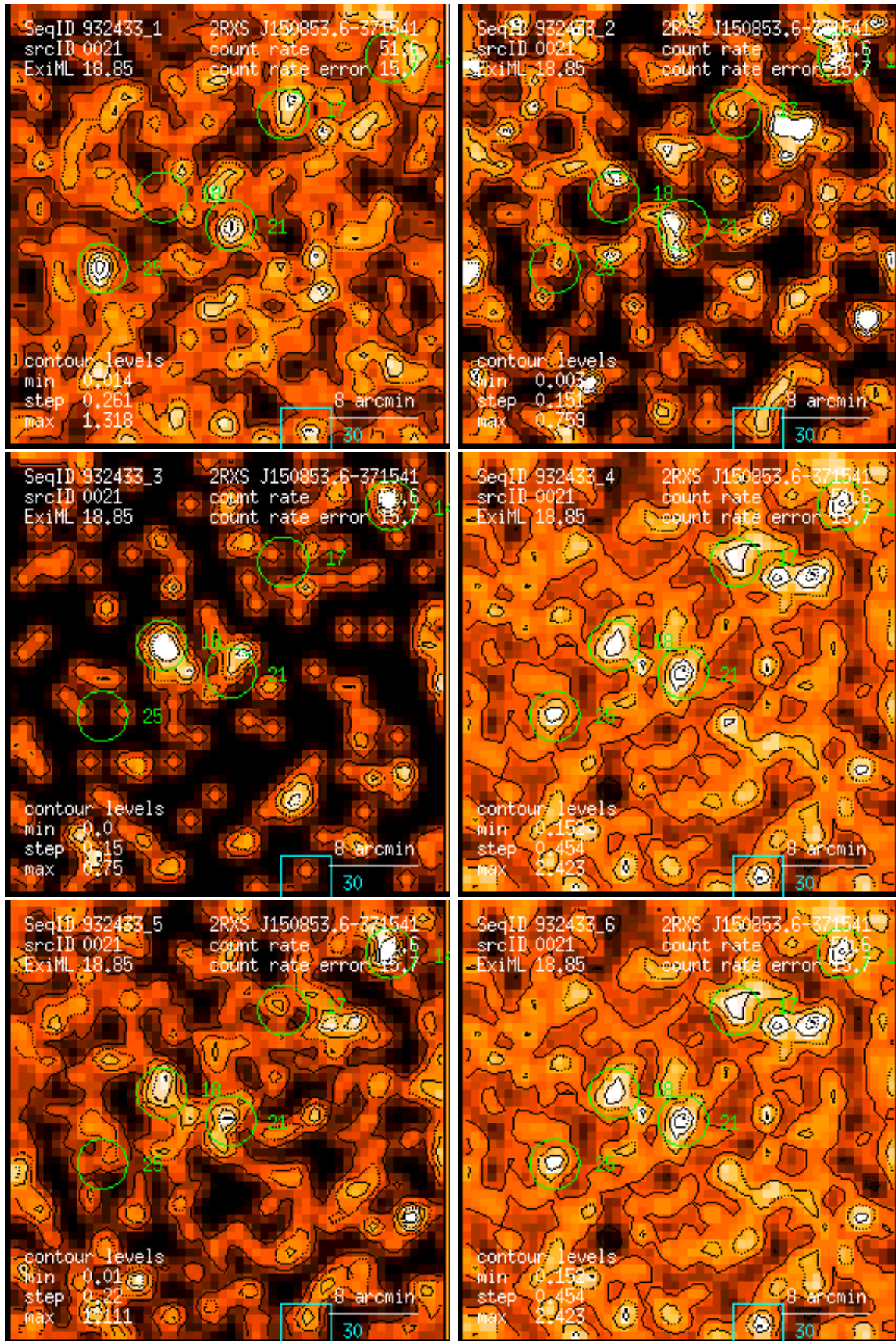
Figure 21: RASS 932433: detection 0021: band rate images, Gaussian filter: (1) PSPC channels 11 – 41, (2) 52 – 90, (3) 91 – 201, (4) 11 – 235, (5) 52 – 201, (6) 11 – 201. Broad band rates in counts/ks. Band rate contour levels in counts/ks/arcmin 2 .
