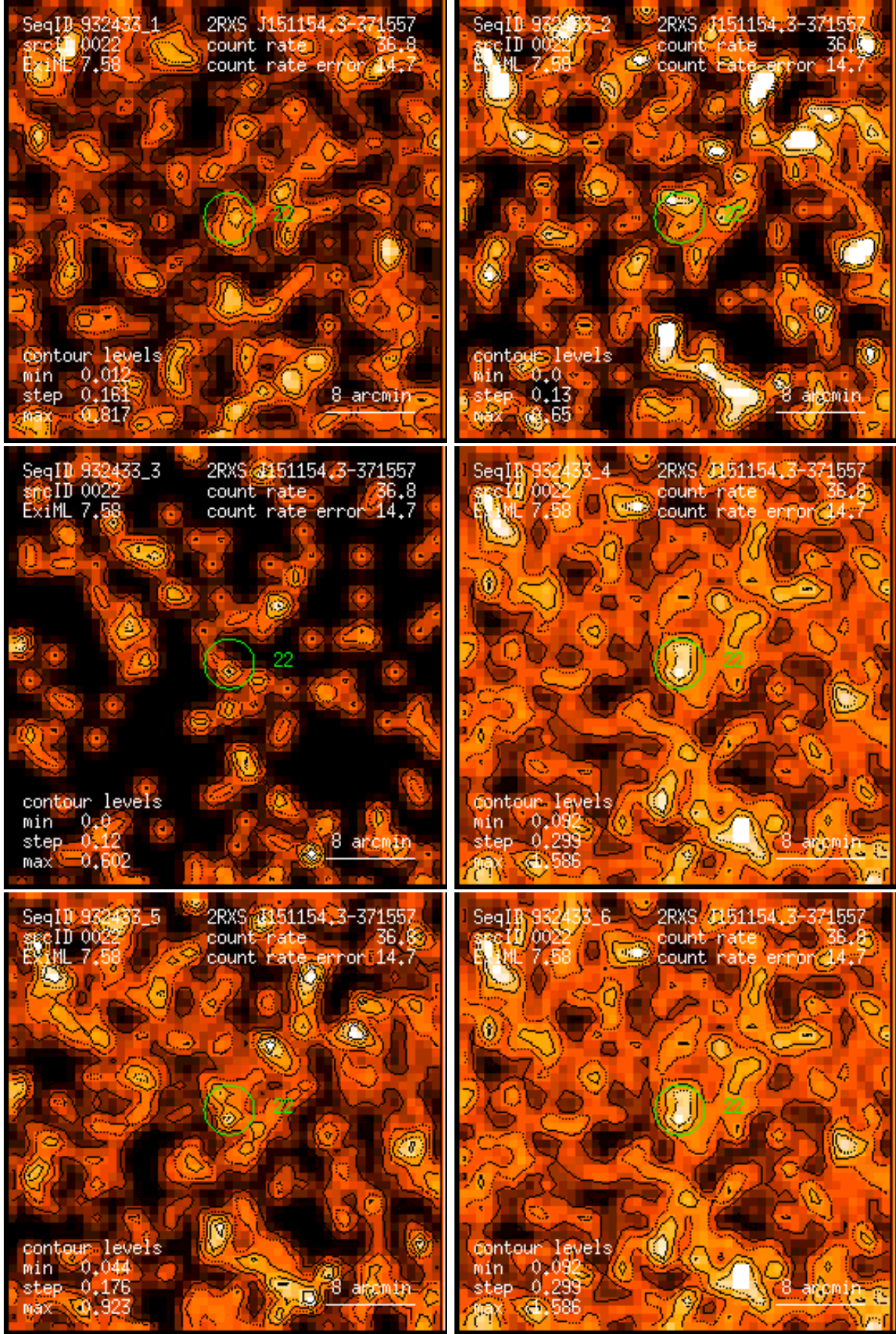
Figure 22: RASS 932433: detection 0022: band rate images, Gaussian filter: (1) PSPC channels 11 – 41, (2) 52 – 90, (3) 91 – 201, (4) 11 – 235, (5) 52 – 201, (6) 11 – 201. Broad band rates in counts/ks. Band rate contour levels in counts/ks/arcmin 2 .
