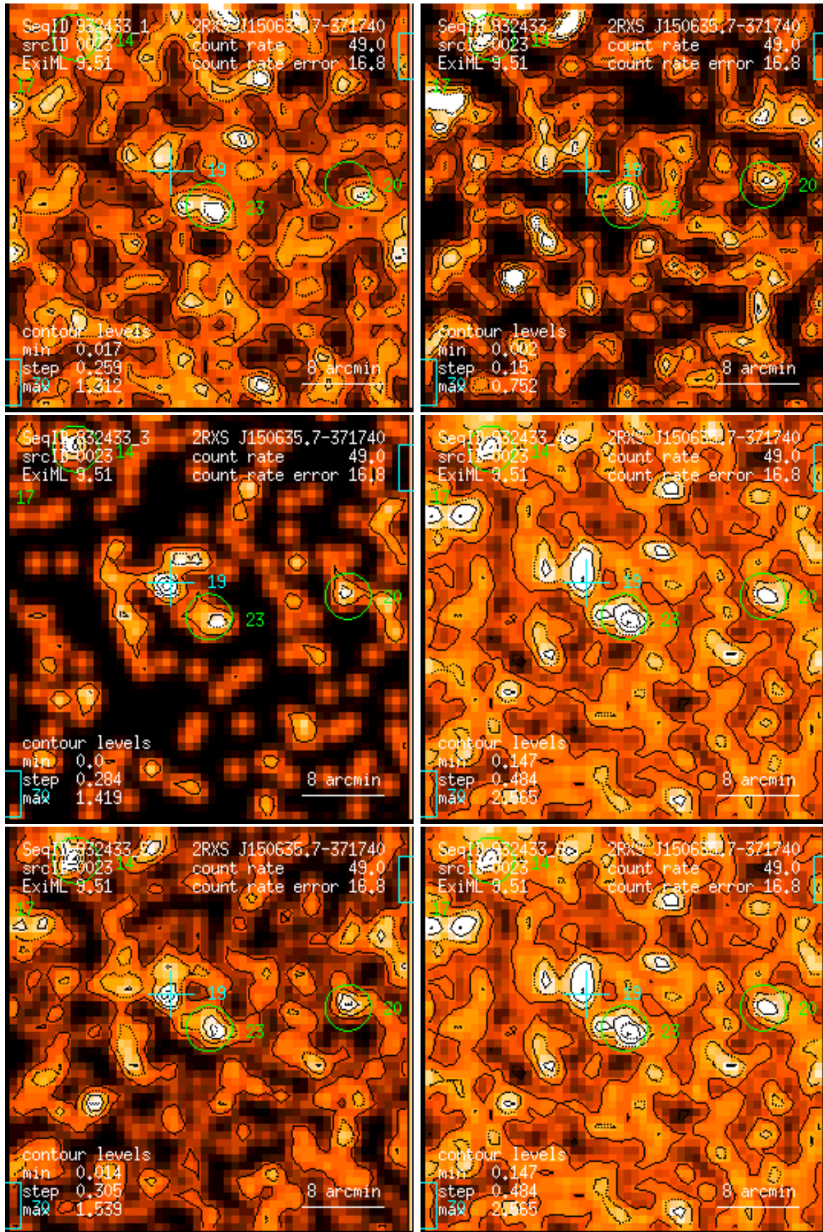
Figure 23: RASS 932433: detection 0023: band rate images, Gaussian filter: (1) PSPC channels 11 – 41, (2) 52 – 90, (3) 91 – 201, (4) 11 – 235, (5) 52 – 201, (6) 11 – 201. Broad band rates in counts/ks. Band rate contour levels in counts/ks/arcmin 2 .
