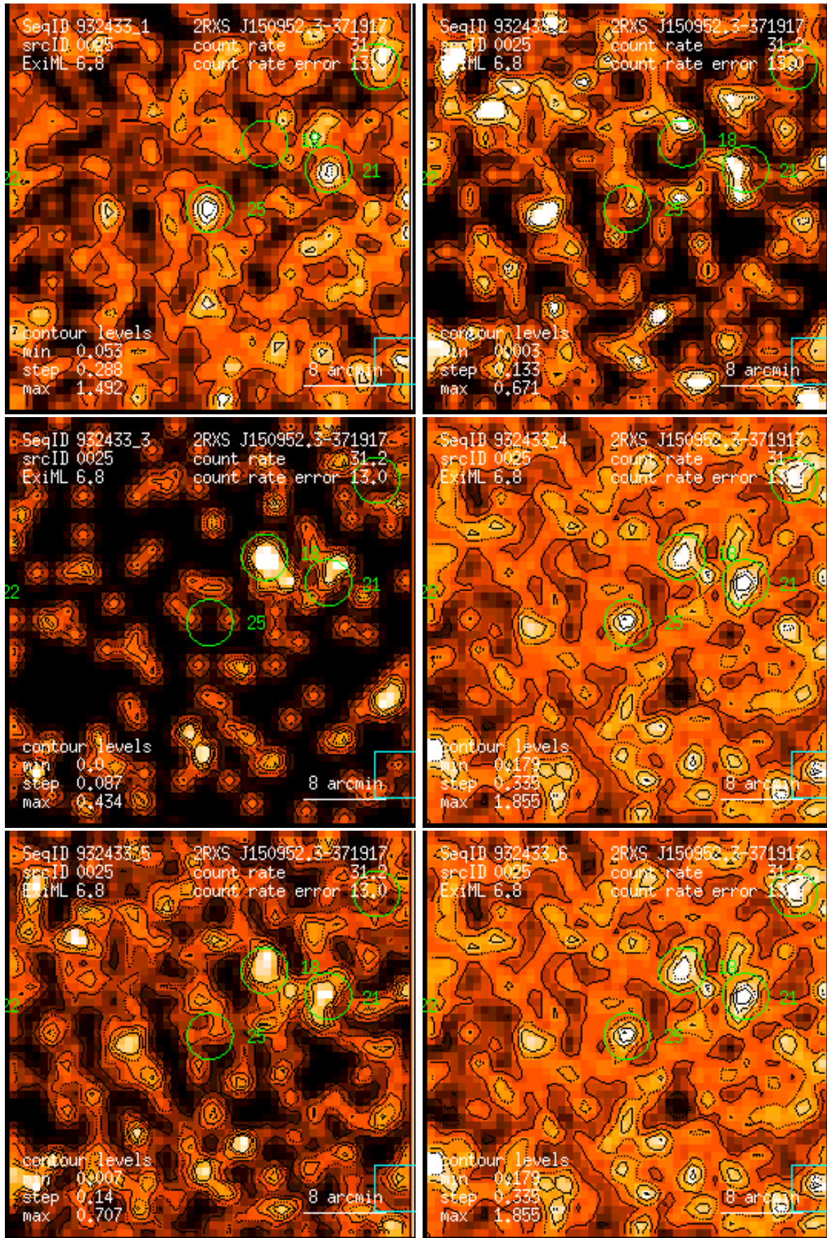
Figure 25: RASS 932433: detection 0025: band rate images, Gaussian filter: (1) PSPC channels 11 – 41, (2) 52 – 90, (3) 91 – 201, (4) 11 – 235, (5) 52 – 201, (6) 11 – 201. Broad band rates in counts/ks. Band rate contour levels in counts/ks/arcmin 2 .
