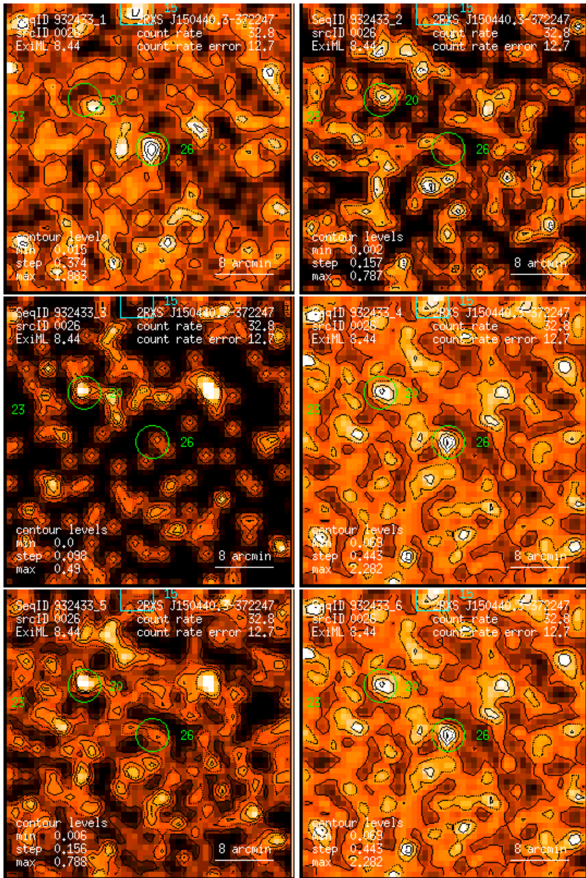
Figure 26: RASS 932433: detection 0026: band rate images, Gaussian filter: (1) PSPC channels 11 – 41, (2) 52 – 90, (3) 91 – 201, (4) 11 – 235, (5) 52 – 201, (6) 11 – 201. Broad band rates in counts/ks. Band rate contour levels in counts/ks/arcmin 2 .
