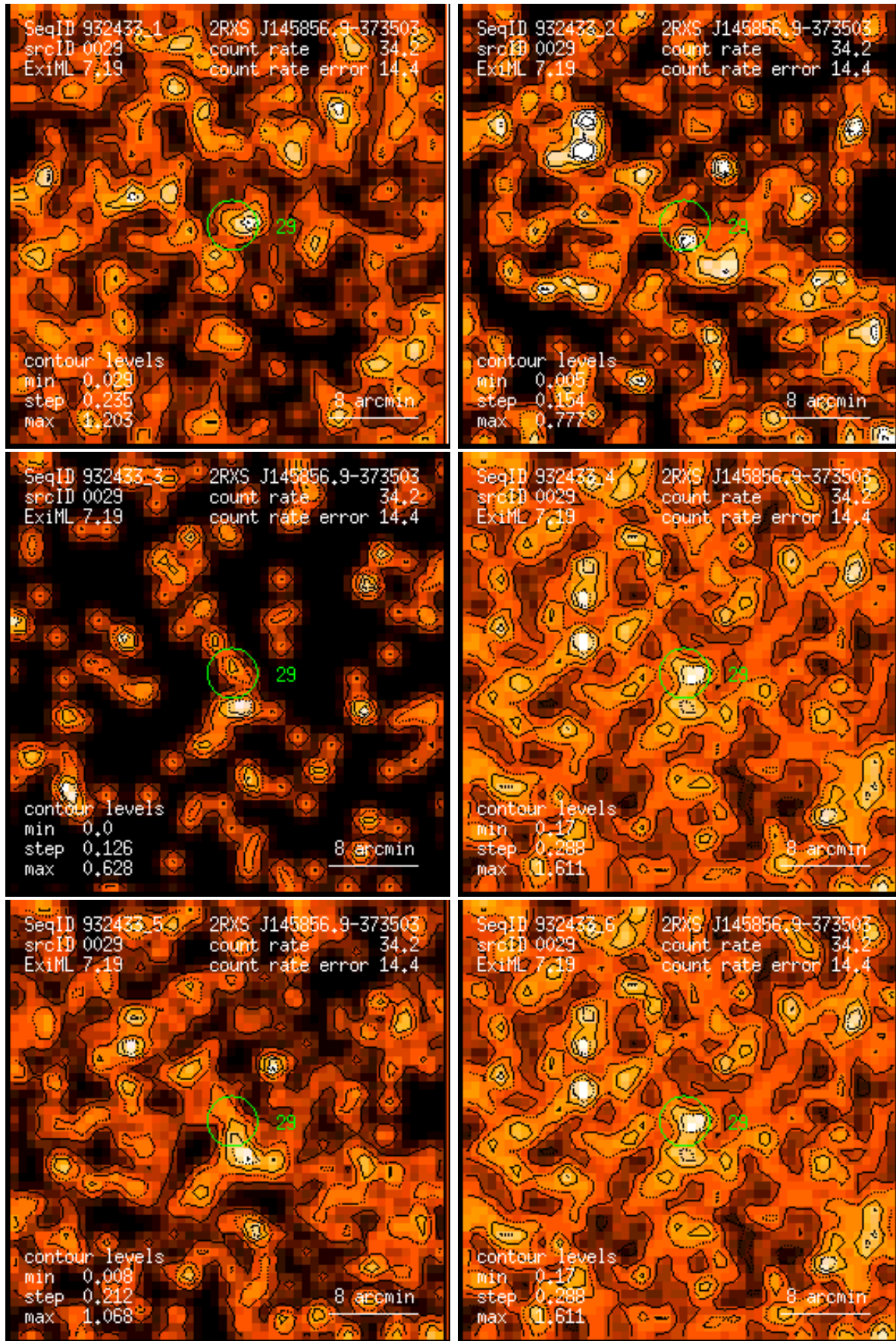
Figure 29: RASS 932433: detection 0029: band rate images, Gaussian filter: (1) PSPC channels 11 – 41, (2) 52 – 90, (3) 91 – 201, (4) 11 – 235, (5) 52 – 201, (6) 11 – 201. Broad band rates in counts/ks. Band rate contour levels in counts/ks/arcmin 2 .
