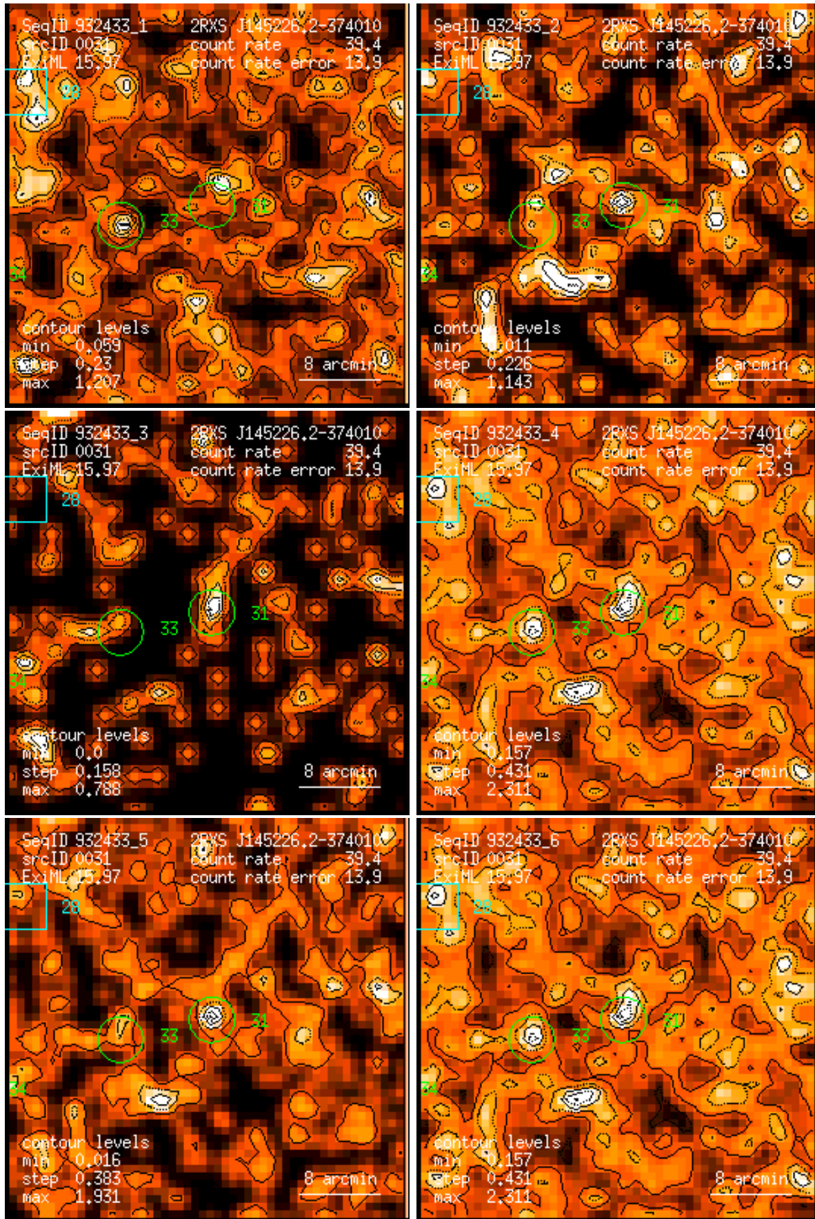
Figure 31: RASS 932433: detection 0031: band rate images, Gaussian filter: (1) PSPC channels 11 – 41, (2) 52 – 90, (3) 91 – 201, (4) 11 – 235, (5) 52 – 201, (6) 11 – 201. Broad band rates in counts/ks. Band rate contour levels in counts/ks/arcmin 2 .
