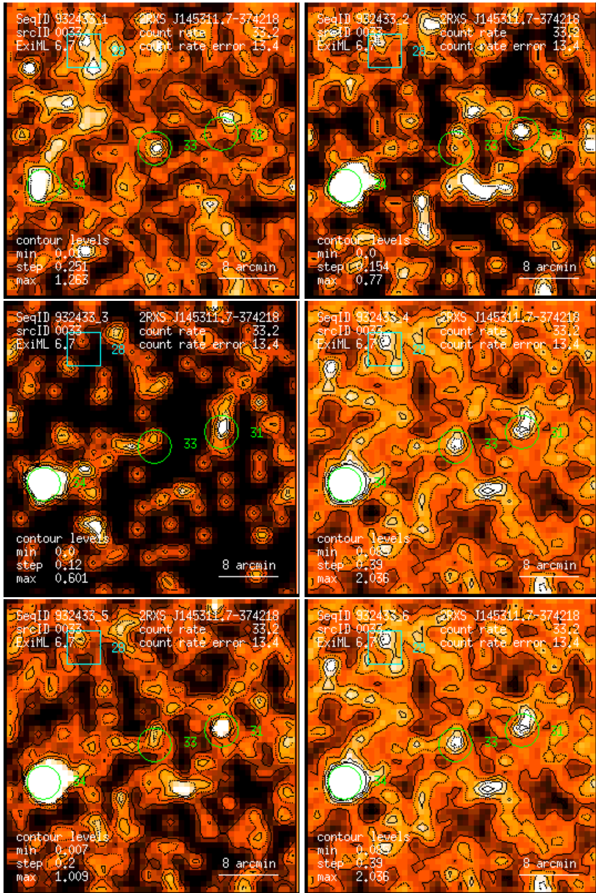
Figure 33: RASS 932433: detection 0033: band rate images, Gaussian filter: (1) PSPC channels 11 – 41, (2) 52 – 90, (3) 91 – 201, (4) 11 – 235, (5) 52 – 201, (6) 11 – 201. Broad band rates in counts/ks. Band rate contour levels in counts/ks/arcmin 2 .
