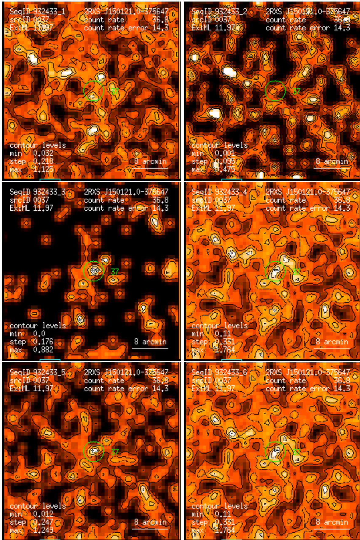
Figure 37: RASS 932433: detection 0037: band rate images, Gaussian filter: (1) PSPC channels 11 – 41, (2) 52 – 90, (3) 91 – 201, (4) 11 – 235, (5) 52 – 201, (6) 11 – 201. Broad band rates in counts/ks. Band rate contour levels in counts/ks/arcmin 2 .
