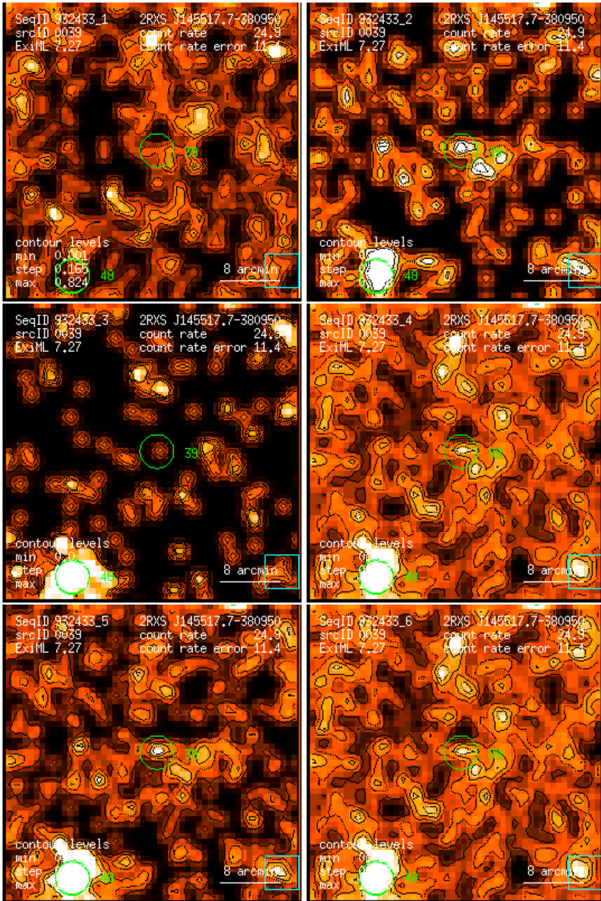
Figure 39: RASS 932433: detection 0039: band rate images, Gaussian filter: (1) PSPC channels 11 – 41, (2) 52 – 90, (3) 91 – 201, (4) 11 – 235, (5) 52 – 201, (6) 11 – 201. Broad band rates in counts/ks. Band rate contour levels in counts/ks/arcmin 2 .
