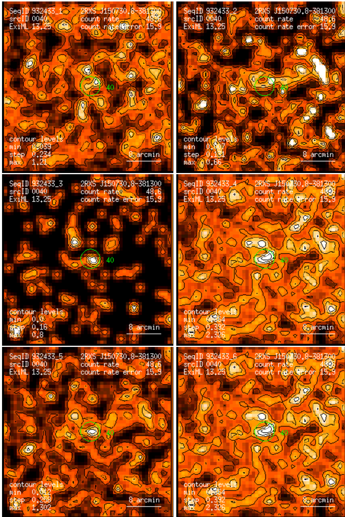
Figure 40: RASS 932433: detection 0040: band rate images, Gaussian filter: (1) PSPC channels 11 – 41, (2) 52 – 90, (3) 91 – 201, (4) 11 – 235, (5) 52 – 201, (6) 11 – 201. Broad band rates in counts/ks. Band rate contour levels in counts/ks/arcmin 2 .
