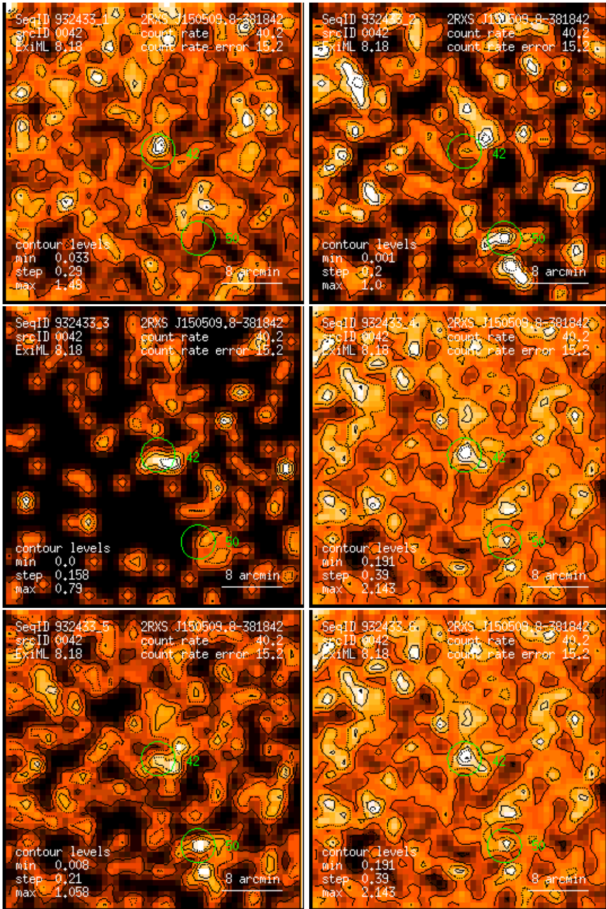
Figure 42: RASS 932433: detection 0042: band rate images, Gaussian filter: (1) PSPC channels 11 – 41, (2) 52 – 90, (3) 91 – 201, (4) 11 – 235, (5) 52 – 201, (6) 11 – 201. Broad band rates in counts/ks. Band rate contour levels in counts/ks/arcmin 2 .
