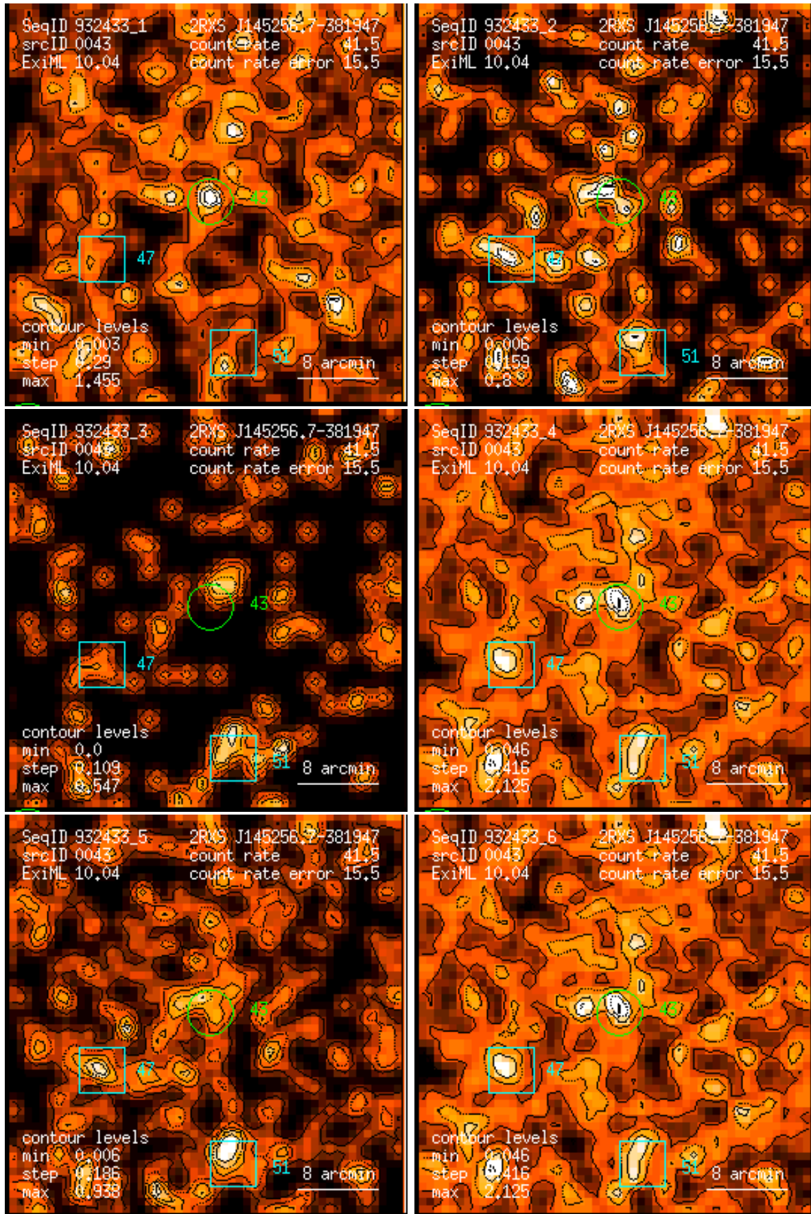
Figure 43: RASS 932433: detection 0043: band rate images, Gaussian filter: (1) PSPC channels 11 – 41, (2) 52 – 90, (3) 91 – 201, (4) 11 – 235, (5) 52 – 201, (6) 11 – 201. Broad band rates in counts/ks. Band rate contour levels in counts/ks/arcmin 2 .
