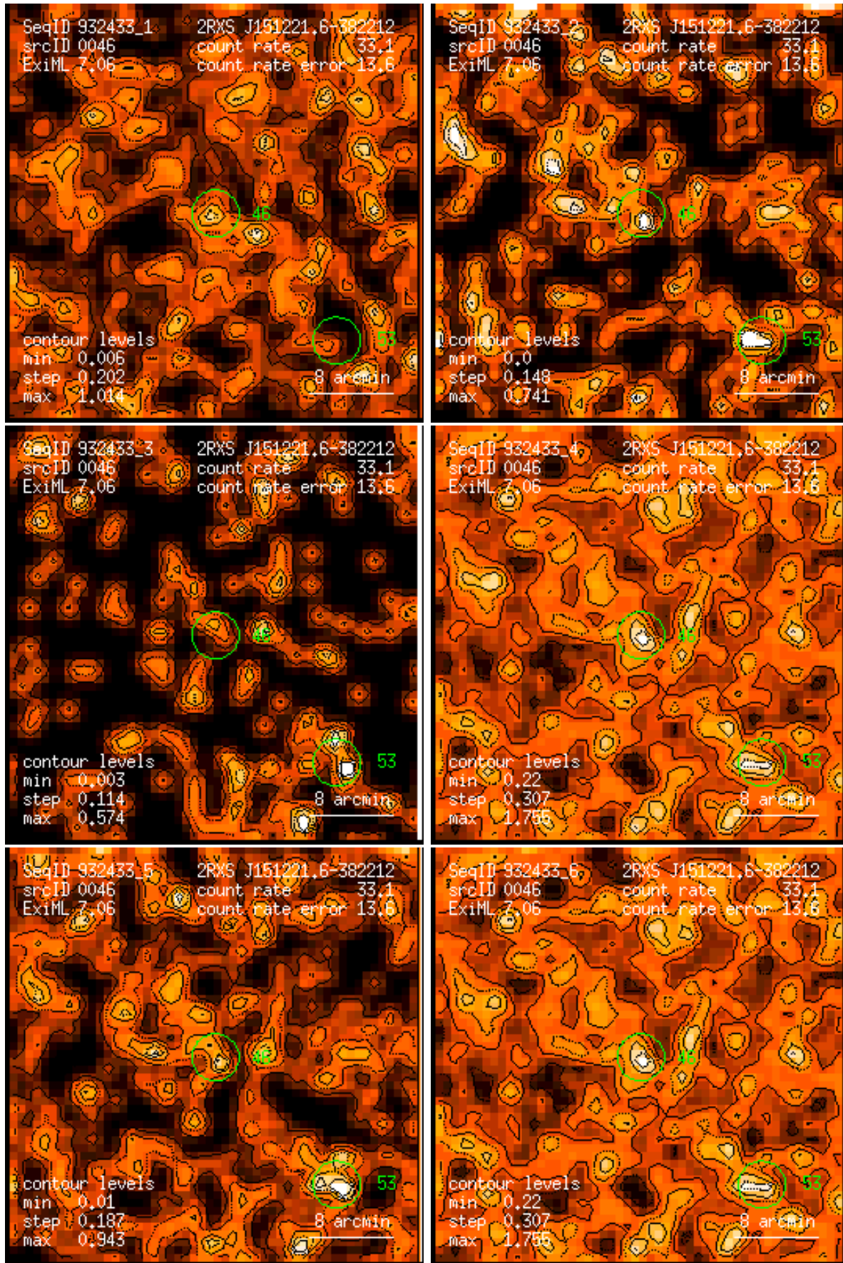
Figure 46: RASS 932433: detection 0046: band rate images, Gaussian filter: (1) PSPC channels 11 – 41, (2) 52 – 90, (3) 91 – 201, (4) 11 – 235, (5) 52 – 201, (6) 11 – 201. Broad band rates in counts/ks. Band rate contour levels in counts/ks/arcmin 2 .
