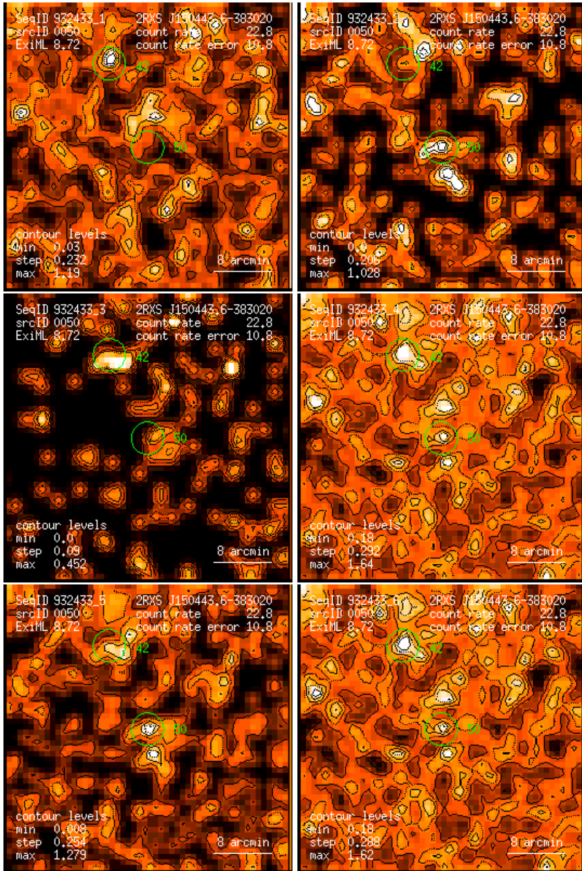
Figure 50: RASS 932433: detection 0050: band rate images, Gaussian filter: (1) PSPC channels 11 – 41, (2) 52 – 90, (3) 91 – 201, (4) 11 – 235, (5) 52 – 201, (6) 11 – 201. Broad band rates in counts/ks. Band rate contour levels in counts/ks/arcmin 2 .
