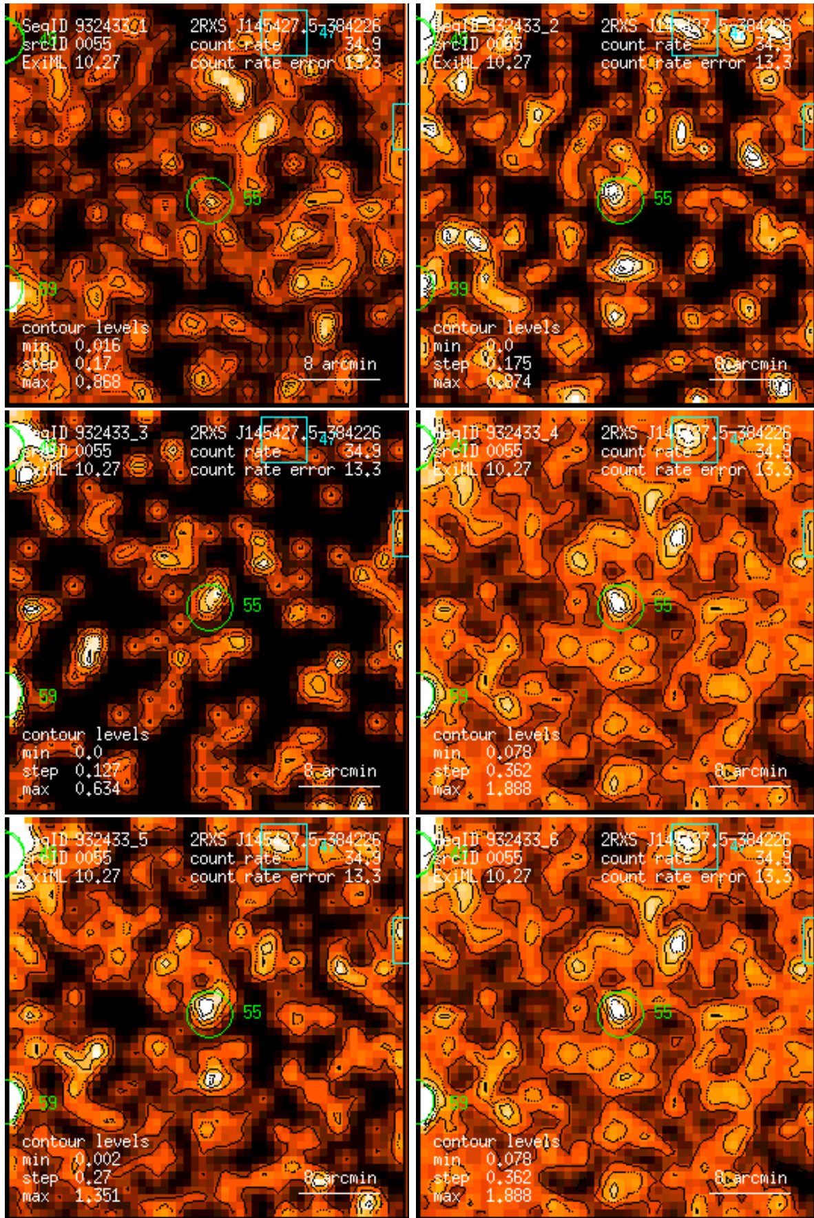
Figure 55: RASS 932433: detection 0055: band rate images, Gaussian filter: (1) PSPC channels 11 – 41, (2) 52 – 90, (3) 91 – 201, (4) 11 – 235, (5) 52 – 201, (6) 11 – 201. Broad band rates in counts/ks. Band rate contour levels in counts/ks/arcmin 2 .
