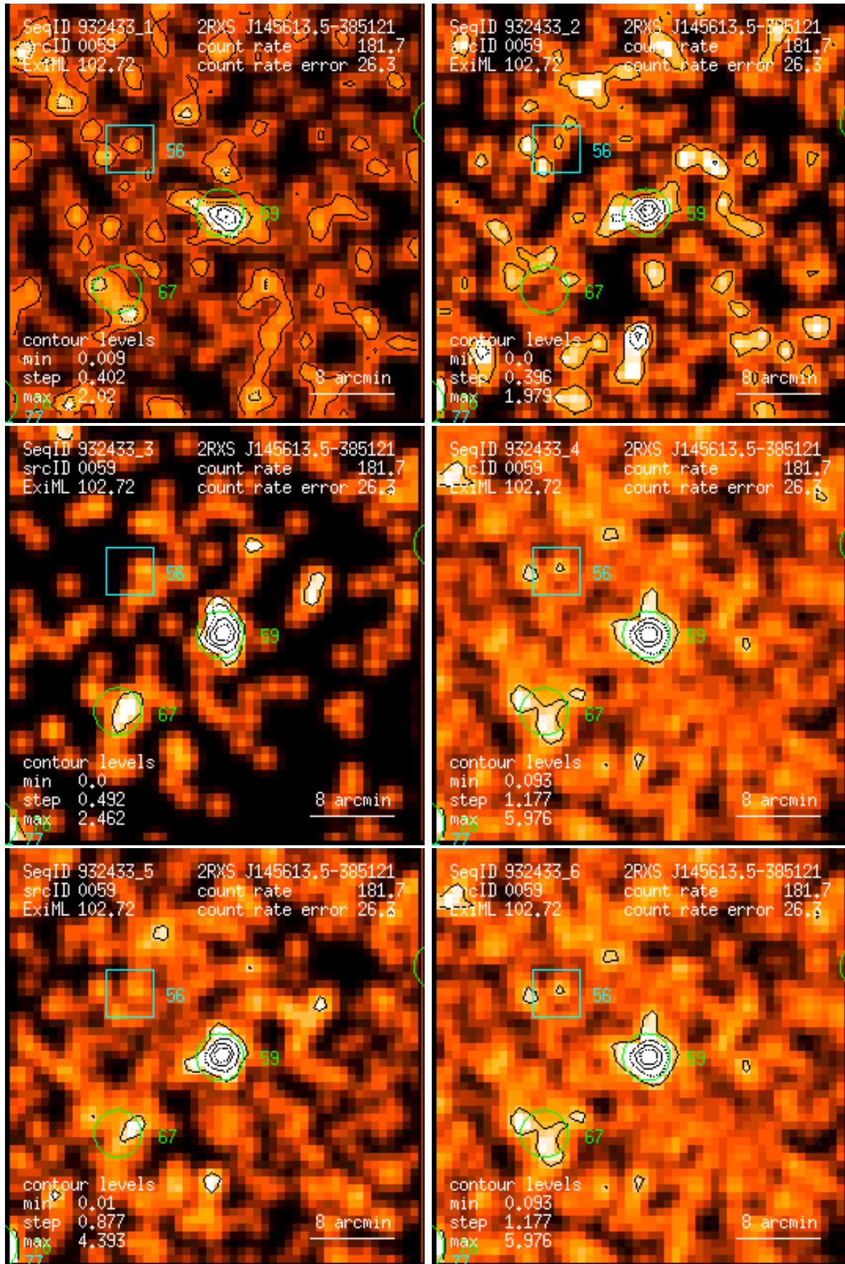
Figure 59: RASS 932433: detection 0059: band rate images, Gaussian filter: (1) PSPC channels 11 – 41, (2) 52 – 90, (3) 91 – 201, (4) 11 – 235, (5) 52 – 201, (6) 11 – 201. Broad band rates in counts/ks. Band rate contour levels in counts/ks/arcmin 2 .
