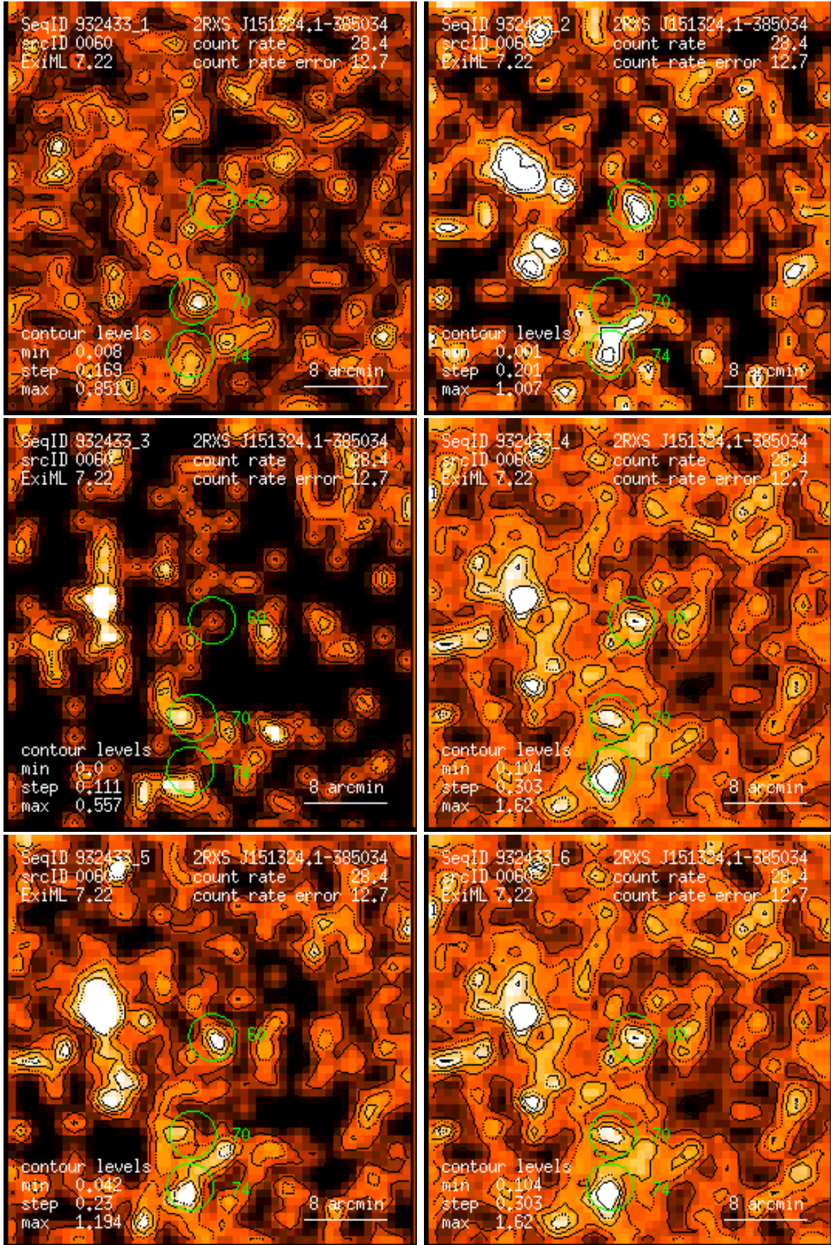
Figure 60: RASS 932433: detection 0060: band rate images, Gaussian filter: (1) PSPC channels 11 – 41, (2) 52 – 90, (3) 91 – 201, (4) 11 – 235, (5) 52 – 201, (6) 11 – 201. Broad band rates in counts/ks. Band rate contour levels in counts/ks/arcmin 2 .
