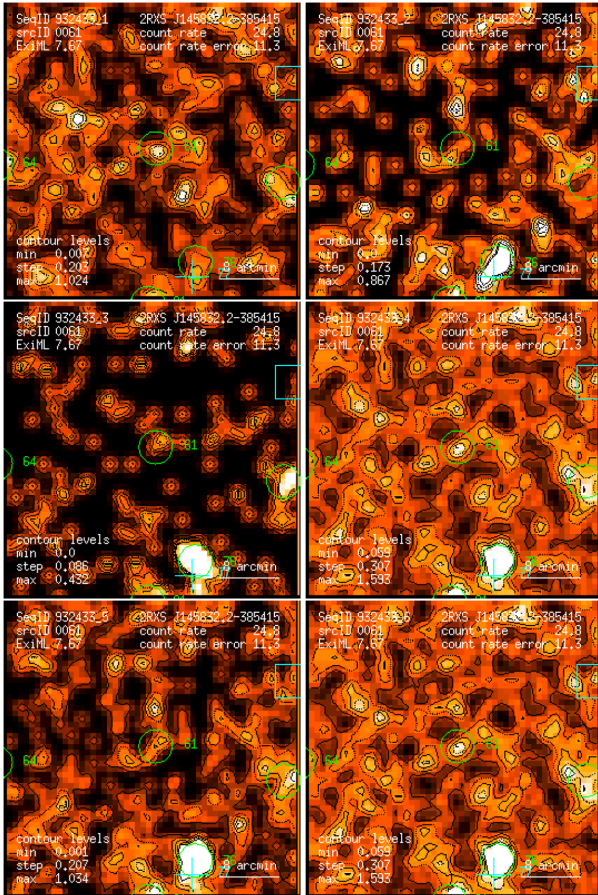
Figure 61: RASS 932433: detection 0061: band rate images, Gaussian filter: (1) PSPC channels 11 – 41, (2) 52 – 90, (3) 91 – 201, (4) 11 – 235, (5) 52 – 201, (6) 11 – 201. Broad band rates in counts/ks. Band rate contour levels in counts/ks/arcmin 2 .
