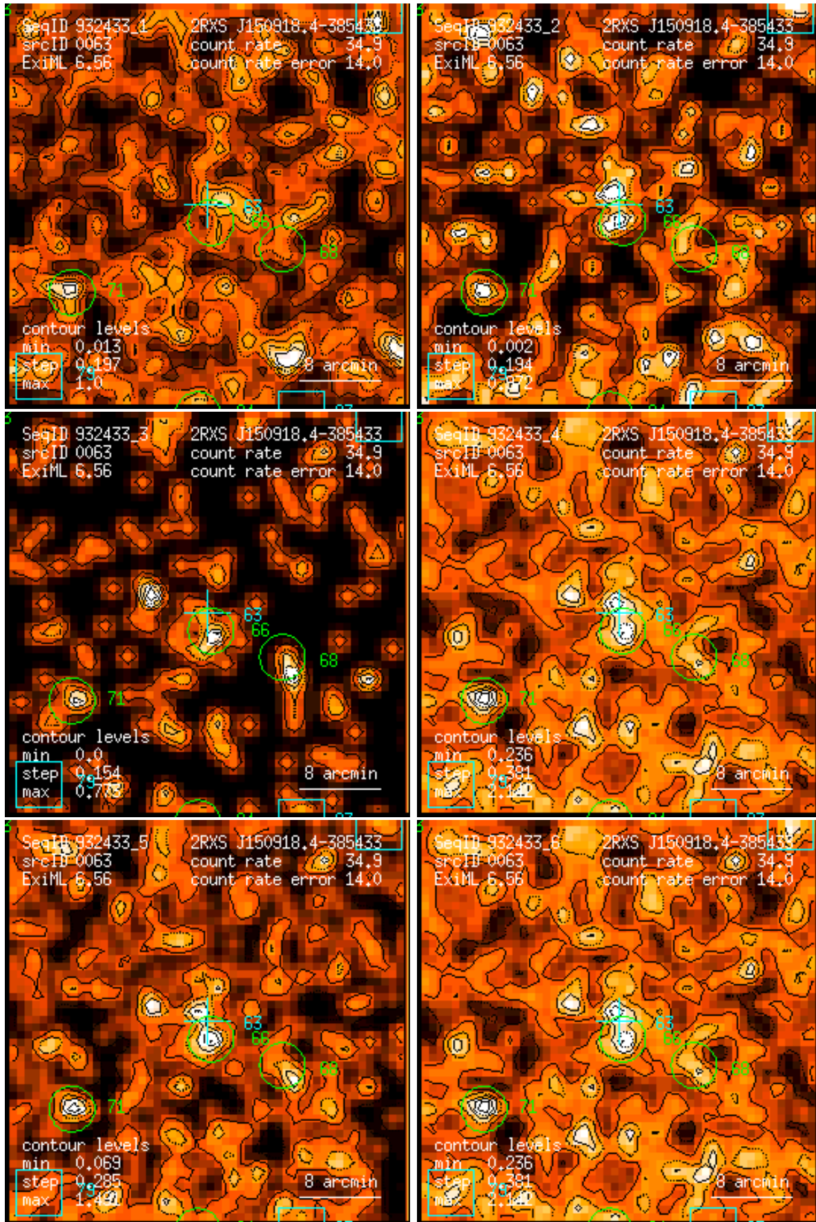
Figure 63: RASS 932433: detection 0063: band rate images, Gaussian filter: (1) PSPC channels 11 – 41, (2) 52 – 90, (3) 91 – 201, (4) 11 – 235, (5) 52 – 201, (6) 11 – 201. Broad band rates in counts/ks. Band rate contour levels in counts/ks/arcmin 2 .
