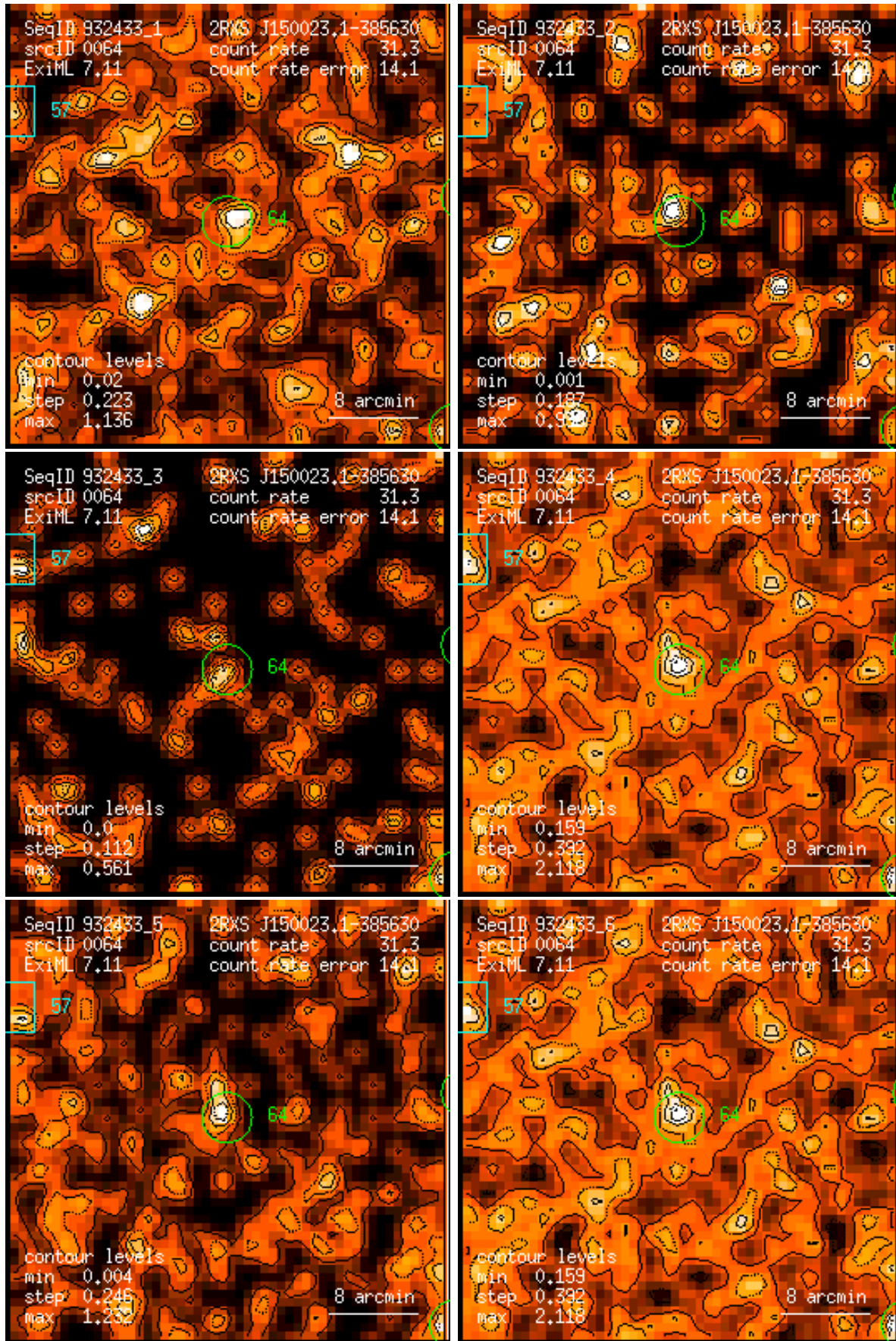
Figure 64: RASS 932433: detection 0064: band rate images, Gaussian filter: (1) PSPC channels 11 – 41, (2) 52 – 90, (3) 91 – 201, (4) 11 – 235, (5) 52 – 201, (6) 11 – 201. Broad band rates in counts/ks. Band rate contour levels in counts/ks/arcmin 2 .
