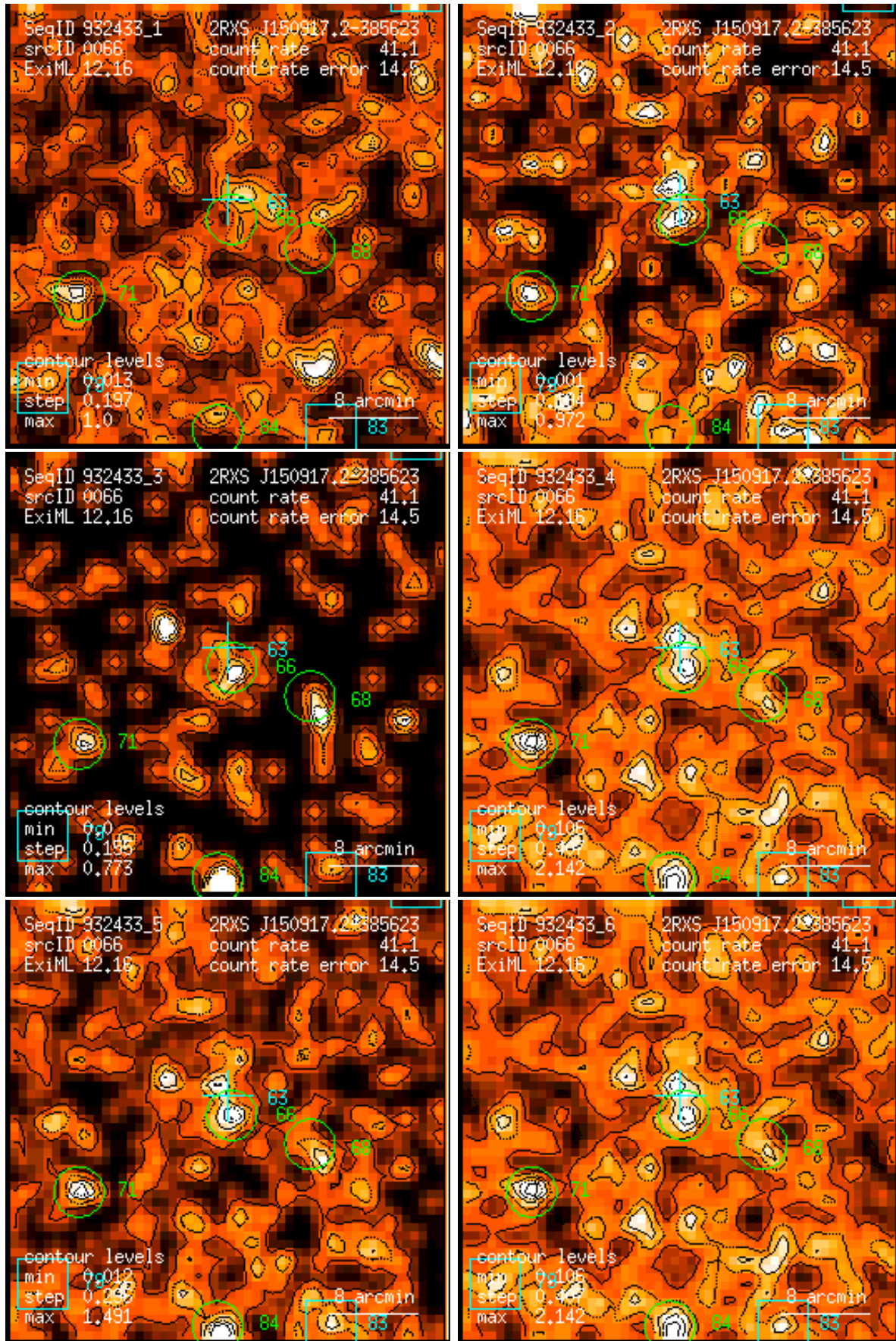
Figure 66: RASS 932433: detection 0066: band rate images, Gaussian filter: (1) PSPC channels 11 – 41, (2) 52 – 90, (3) 91 – 201, (4) 11 – 235, (5) 52 – 201, (6) 11 – 201. Broad band rates in counts/ks. Band rate contour levels in counts/ks/arcmin 2 .
