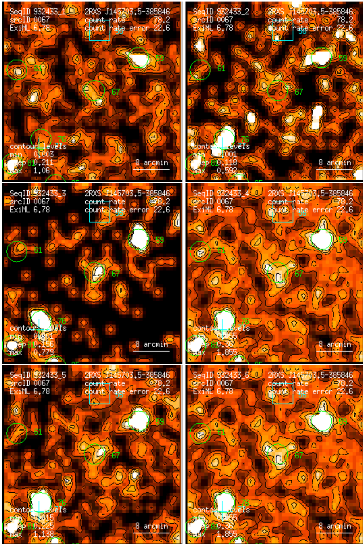
Figure 67: RASS 932433: detection 0067: band rate images, Gaussian filter: (1) PSPC channels 11 – 41, (2) 52 – 90, (3) 91 – 201, (4) 11 – 235, (5) 52 – 201, (6) 11 – 201. Broad band rates in counts/ks. Band rate contour levels in counts/ks/arcmin 2 .
