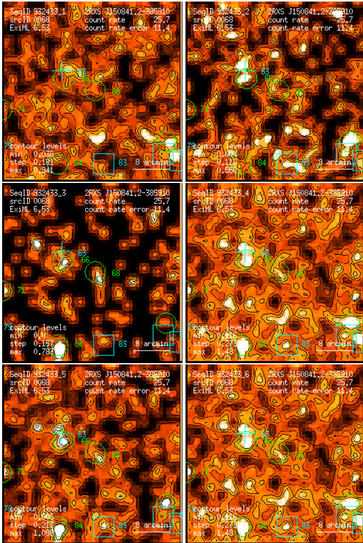
Figure 68: RASS 932433: detection 0068: band rate images, Gaussian filter: (1) PSPC channels 11 – 41, (2) 52 – 90, (3) 91 – 201, (4) 11 – 235, (5) 52 – 201, (6) 11 – 201. Broad band rates in counts/ks. Band rate contour levels in counts/ks/arcmin 2 .
