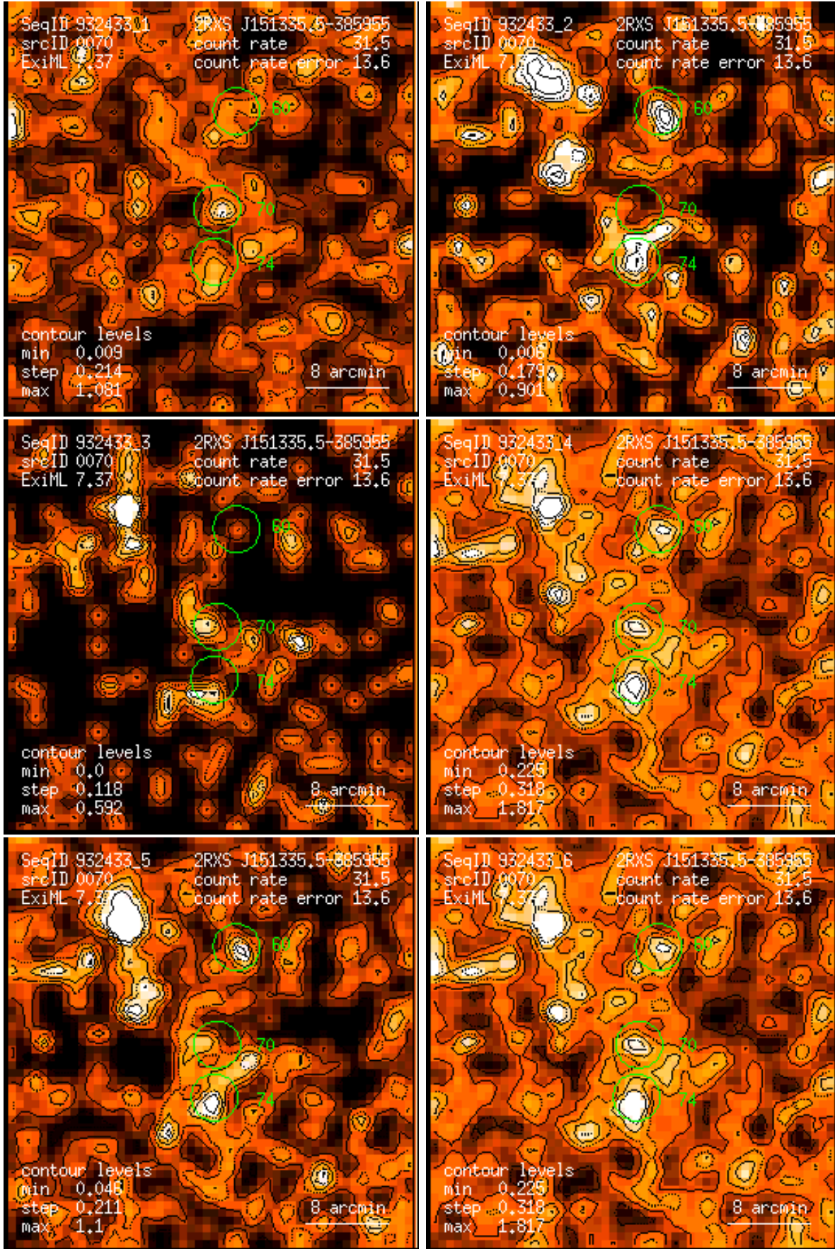
Figure 70: RASS 932433: detection 0070: band rate images, Gaussian filter: (1) PSPC channels 11 – 41, (2) 52 – 90, (3) 91 – 201, (4) 11 – 235, (5) 52 – 201, (6) 11 – 201. Broad band rates in counts/ks. Band rate contour levels in counts/ks/arcmin 2 .
