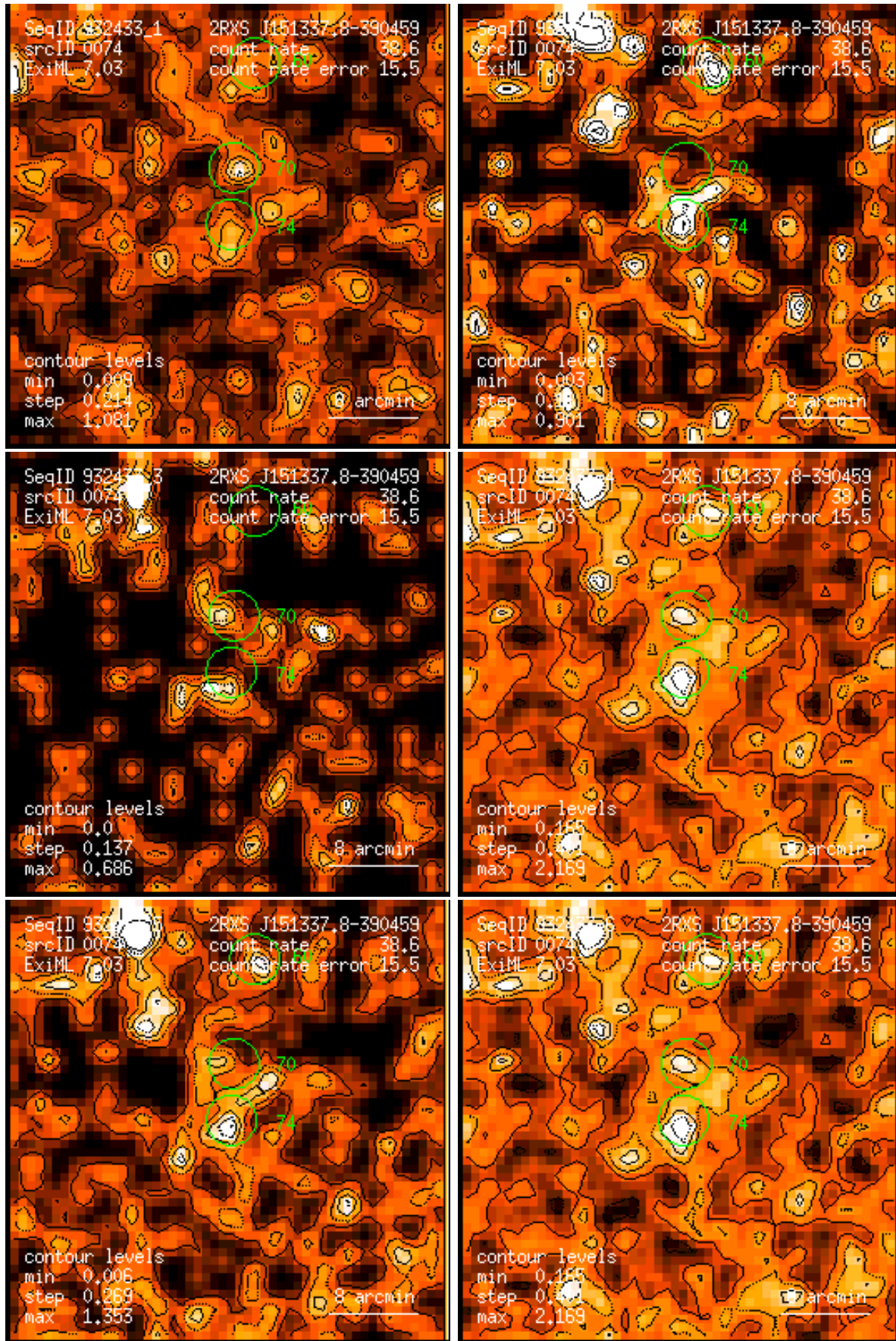
Figure 74: RASS 932433: detection 0074: band rate images, Gaussian filter: (1) PSPC channels 11 – 41, (2) 52 – 90, (3) 91 – 201, (4) 11 – 235, (5) 52 – 201, (6) 11 – 201. Broad band rates in counts/ks. Band rate contour levels in counts/ks/arcmin 2 .
