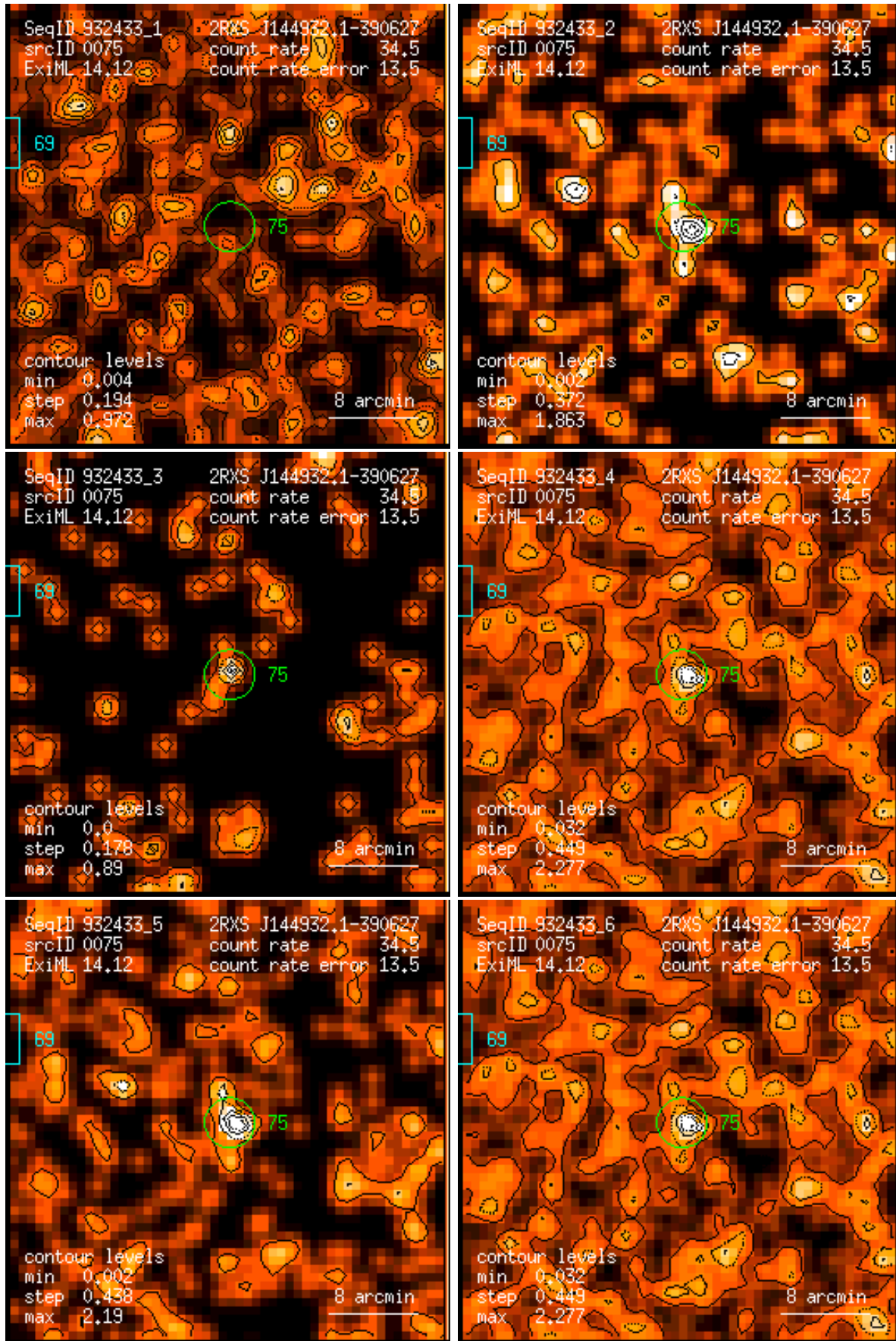
Figure 75: RASS 932433: detection 0075: band rate images, Gaussian filter: (1) PSPC channels 11 – 41, (2) 52 – 90, (3) 91 – 201, (4) 11 – 235, (5) 52 – 201, (6) 11 – 201. Broad band rates in counts/ks. Band rate contour levels in counts/ks/arcmin 2 .
