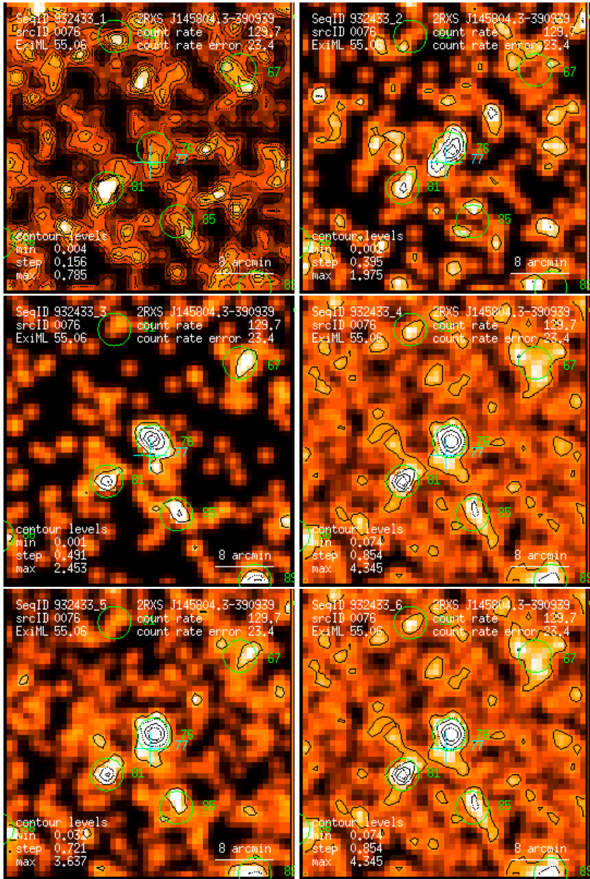
Figure 76: RASS 932433: detection 0076: band rate images, Gaussian filter: (1) PSPC channels 11 – 41, (2) 52 – 90, (3) 91 – 201, (4) 11 – 235, (5) 52 – 201, (6) 11 – 201. Broad band rates in counts/ks. Band rate contour levels in counts/ks/arcmin 2 .
