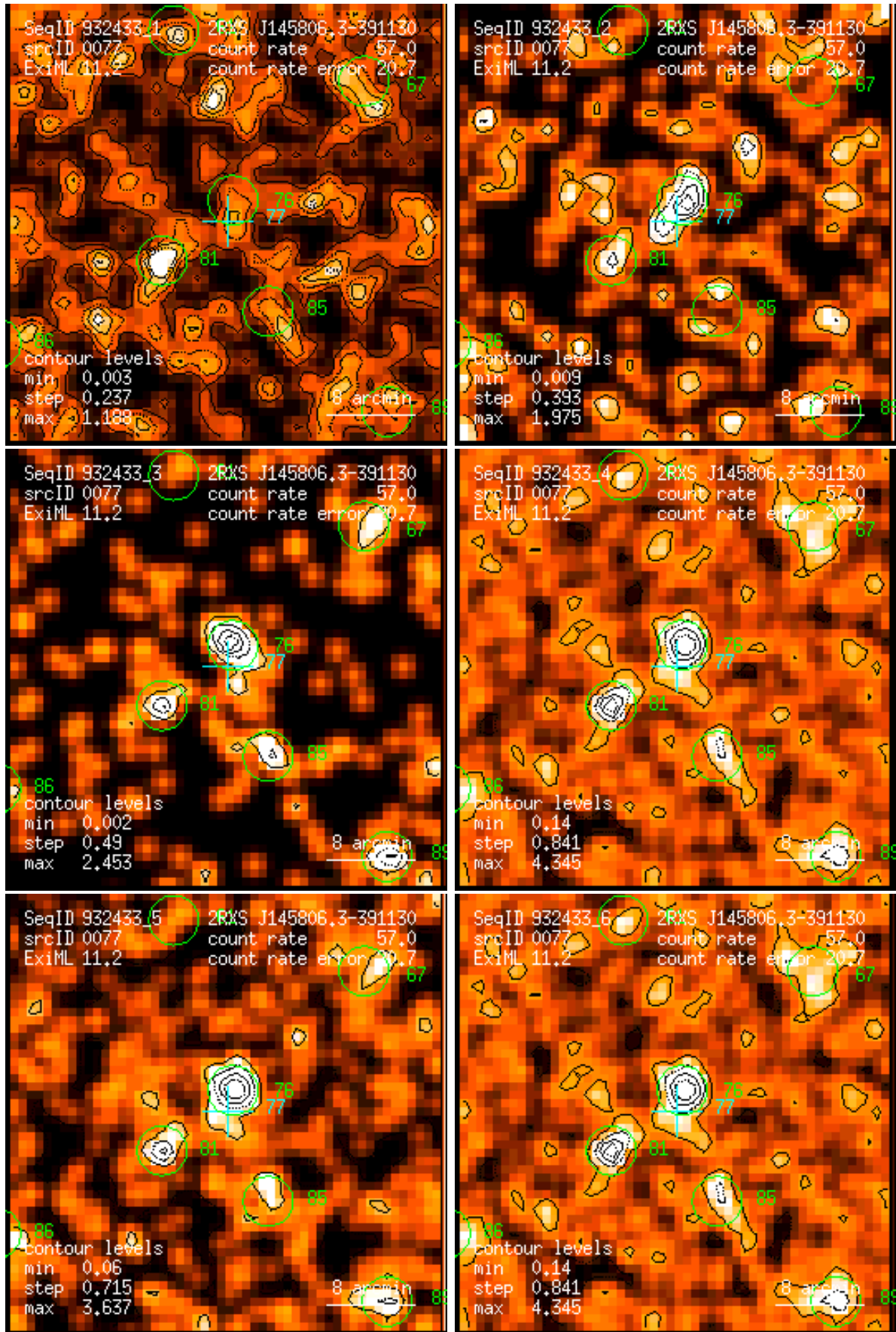
Figure 77: RASS 932433: detection 0077: band rate images, Gaussian filter: (1) PSPC channels 11 – 41, (2) 52 – 90, (3) 91 – 201, (4) 11 – 235, (5) 52 – 201, (6) 11 – 201. Broad band rates in counts/ks. Band rate contour levels in counts/ks/arcmin 2 .
