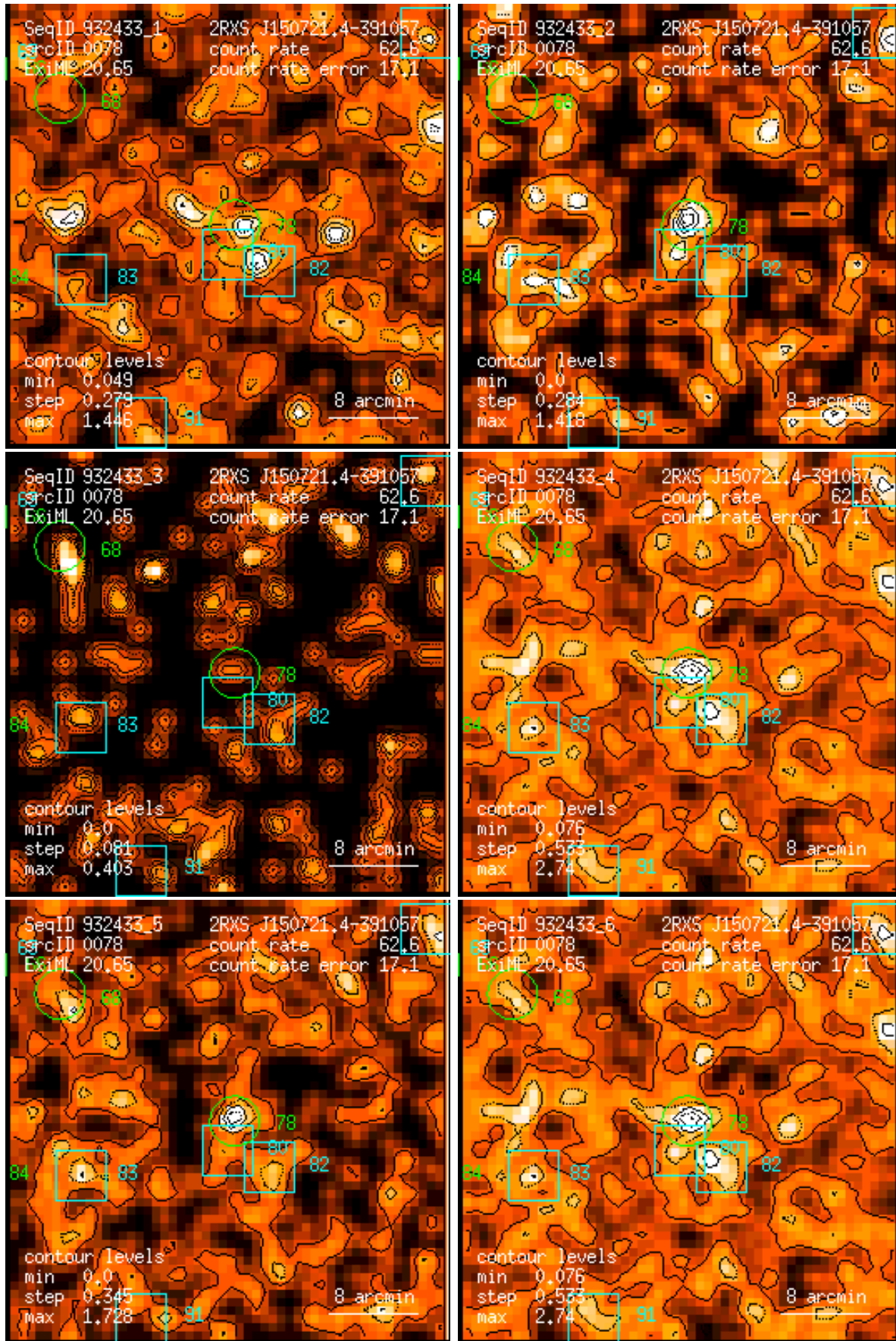
Figure 78: RASS 932433: detection 0078: band rate images, Gaussian filter: (1) PSPC channels 11 – 41, (2) 52 – 90, (3) 91 – 201, (4) 11 – 235, (5) 52 – 201, (6) 11 – 201. Broad band rates in counts/ks. Band rate contour levels in counts/ks/arcmin 2 .
