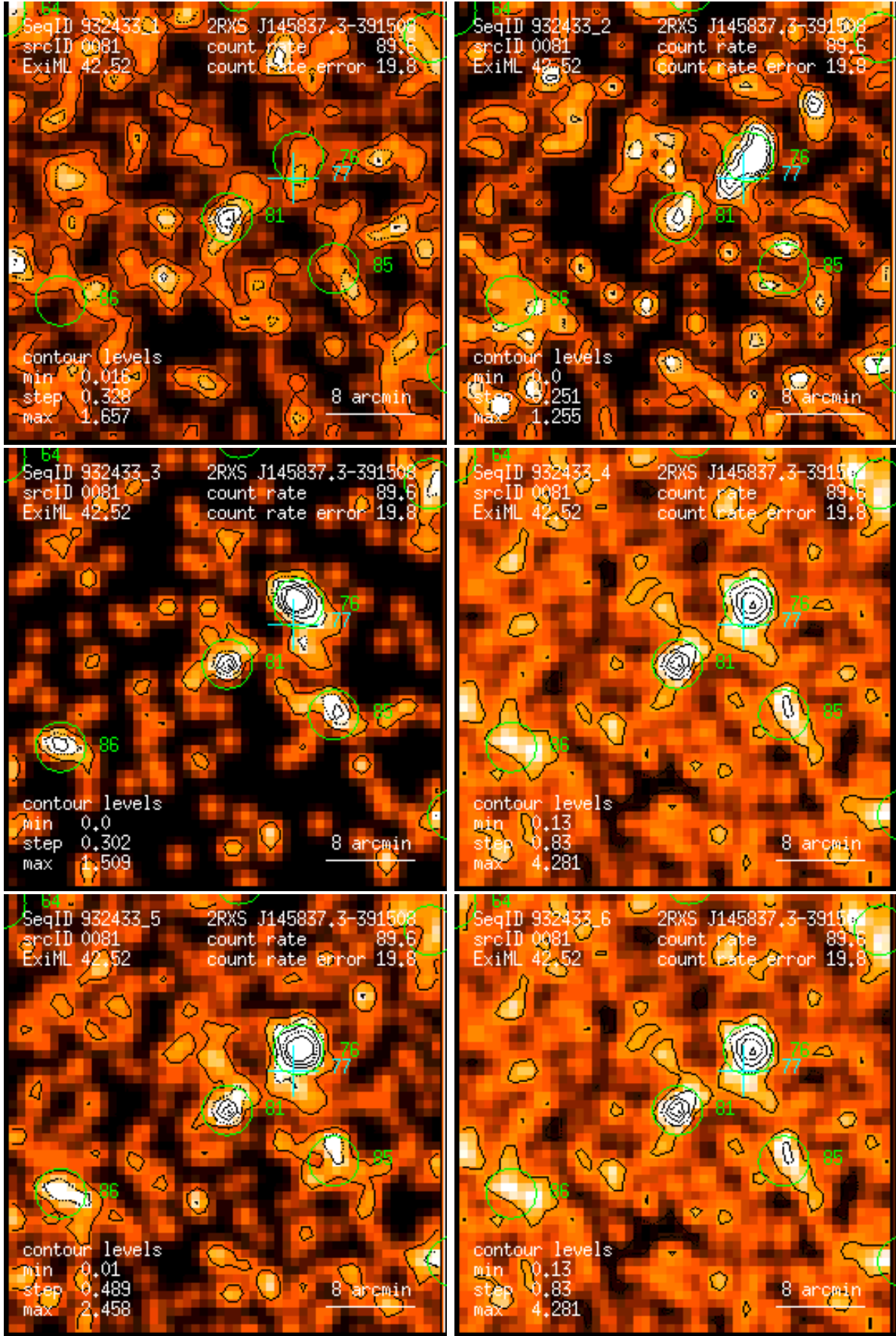
Figure 81: RASS 932433: detection 0081: band rate images, Gaussian filter: (1) PSPC channels 11 – 41, (2) 52 – 90, (3) 91 – 201, (4) 11 – 235, (5) 52 – 201, (6) 11 – 201. Broad band rates in counts/ks. Band rate contour levels in counts/ks/arcmin 2 .
