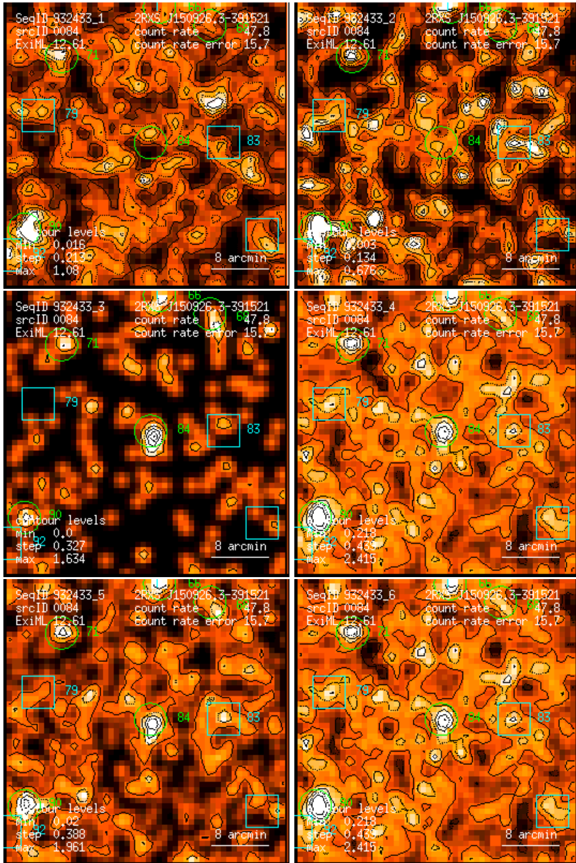
Figure 84: RASS 932433: detection 0084: band rate images, Gaussian filter: (1) PSPC channels 11 – 41, (2) 52 – 90, (3) 91 – 201, (4) 11 – 235, (5) 52 – 201, (6) 11 – 201. Broad band rates in counts/ks. Band rate contour levels in counts/ks/arcmin 2 .
