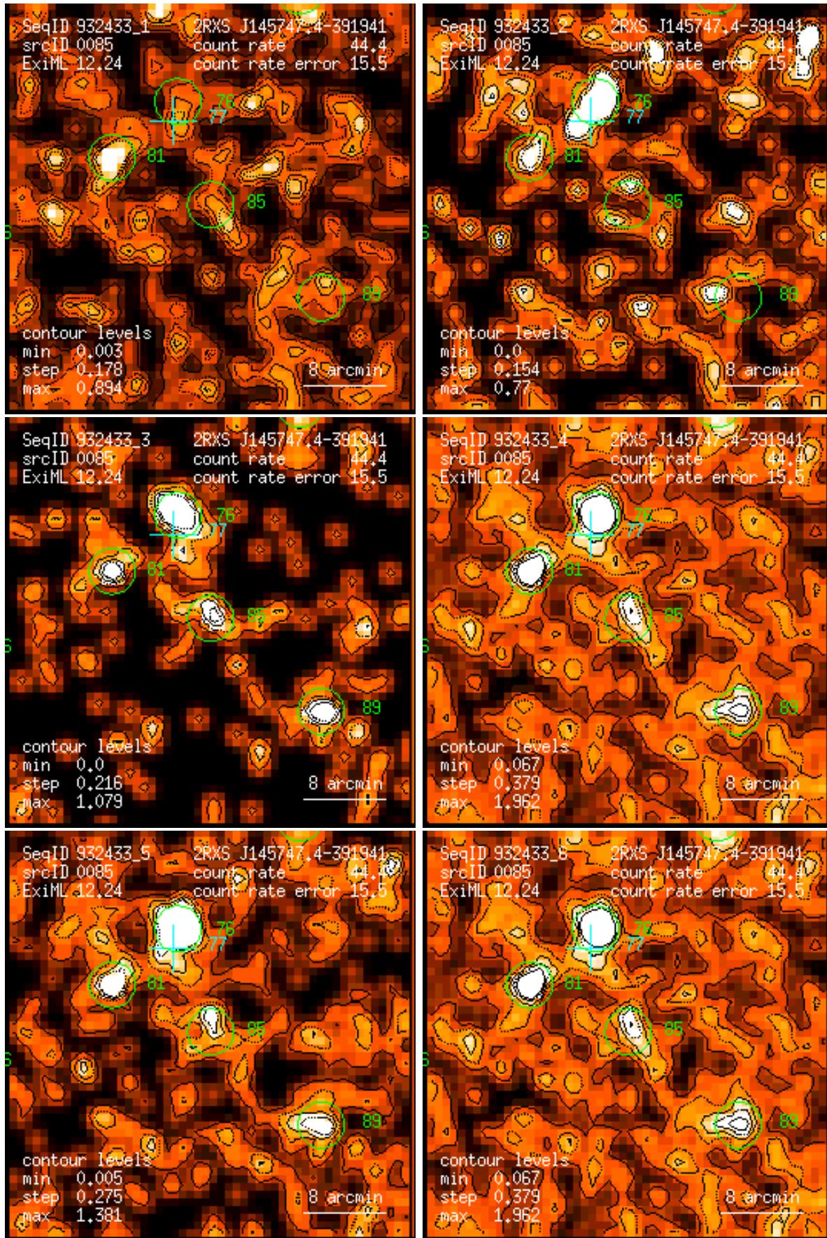
Figure 85: RASS 932433: detection 0085: band rate images, Gaussian filter: (1) PSPC channels 11 – 41, (2) 52 – 90, (3) 91 – 201, (4) 11 – 235, (5) 52 – 201, (6) 11 – 201. Broad band rates in counts/ks. Band rate contour levels in counts/ks/arcmin 2 .
