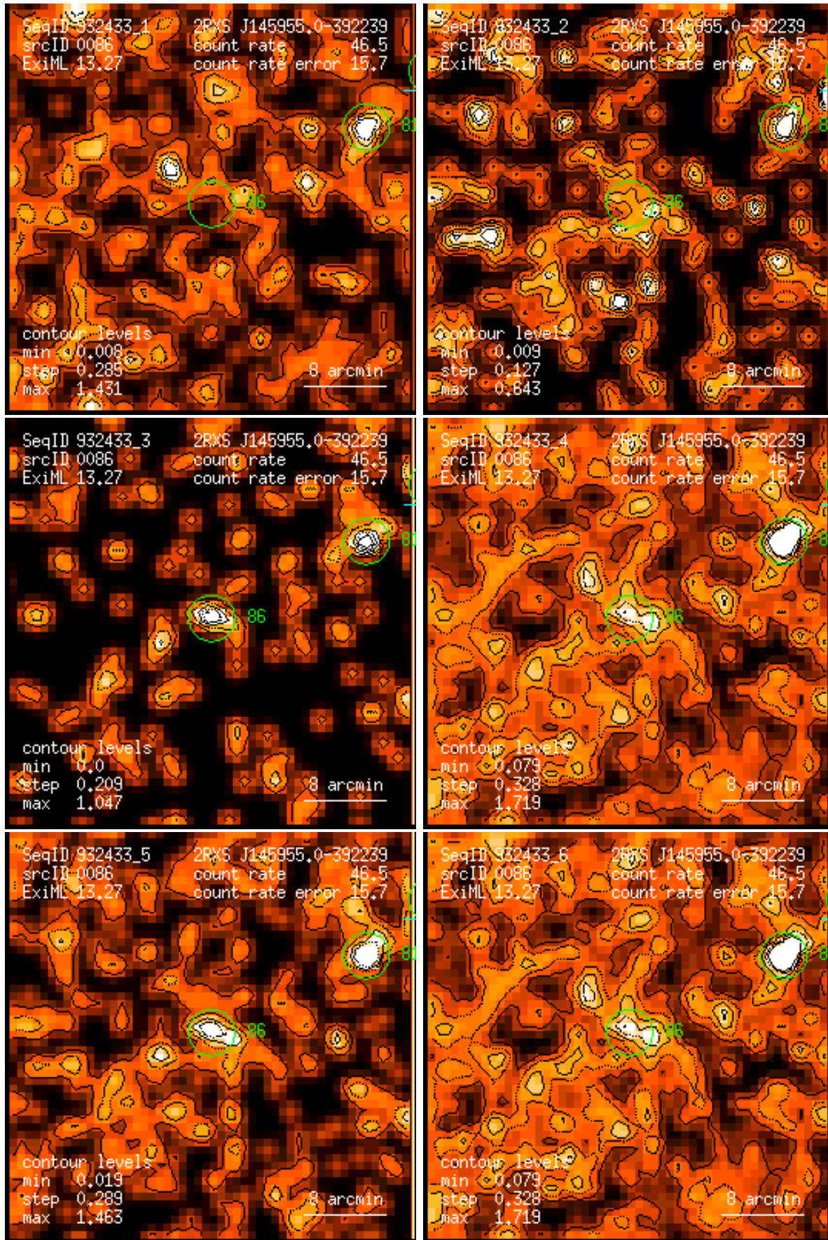
Figure 86: RASS 932433: detection 0086: band rate images, Gaussian filter: (1) PSPC channels 11 – 41, (2) 52 – 90, (3) 91 – 201, (4) 11 – 235, (5) 52 – 201, (6) 11 – 201. Broad band rates in counts/ks. Band rate contour levels in counts/ks/arcmin 2 .
