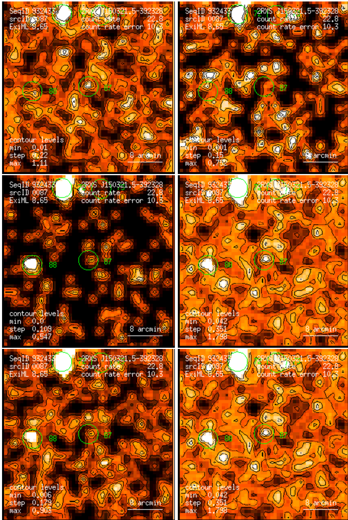
Figure 87: RASS 932433: detection 0087: band rate images, Gaussian filter: (1) PSPC channels 11 – 41, (2) 52 – 90, (3) 91 – 201, (4) 11 – 235, (5) 52 – 201, (6) 11 – 201. Broad band rates in counts/ks. Band rate contour levels in counts/ks/arcmin 2 .
