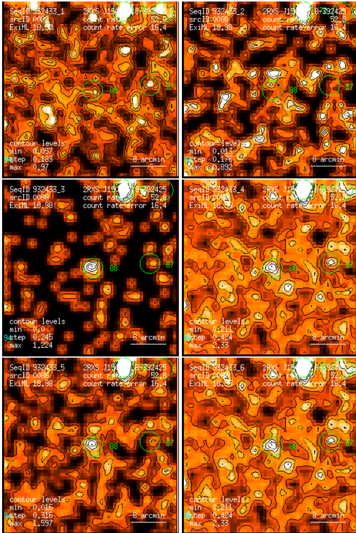
Figure 88: RASS 932433: detection 0088: band rate images, Gaussian filter: (1) PSPC channels 11 – 41, (2) 52 – 90, (3) 91 – 201, (4) 11 – 235, (5) 52 – 201, (6) 11 – 201. Broad band rates in counts/ks. Band rate contour levels in counts/ks/arcmin 2 .
