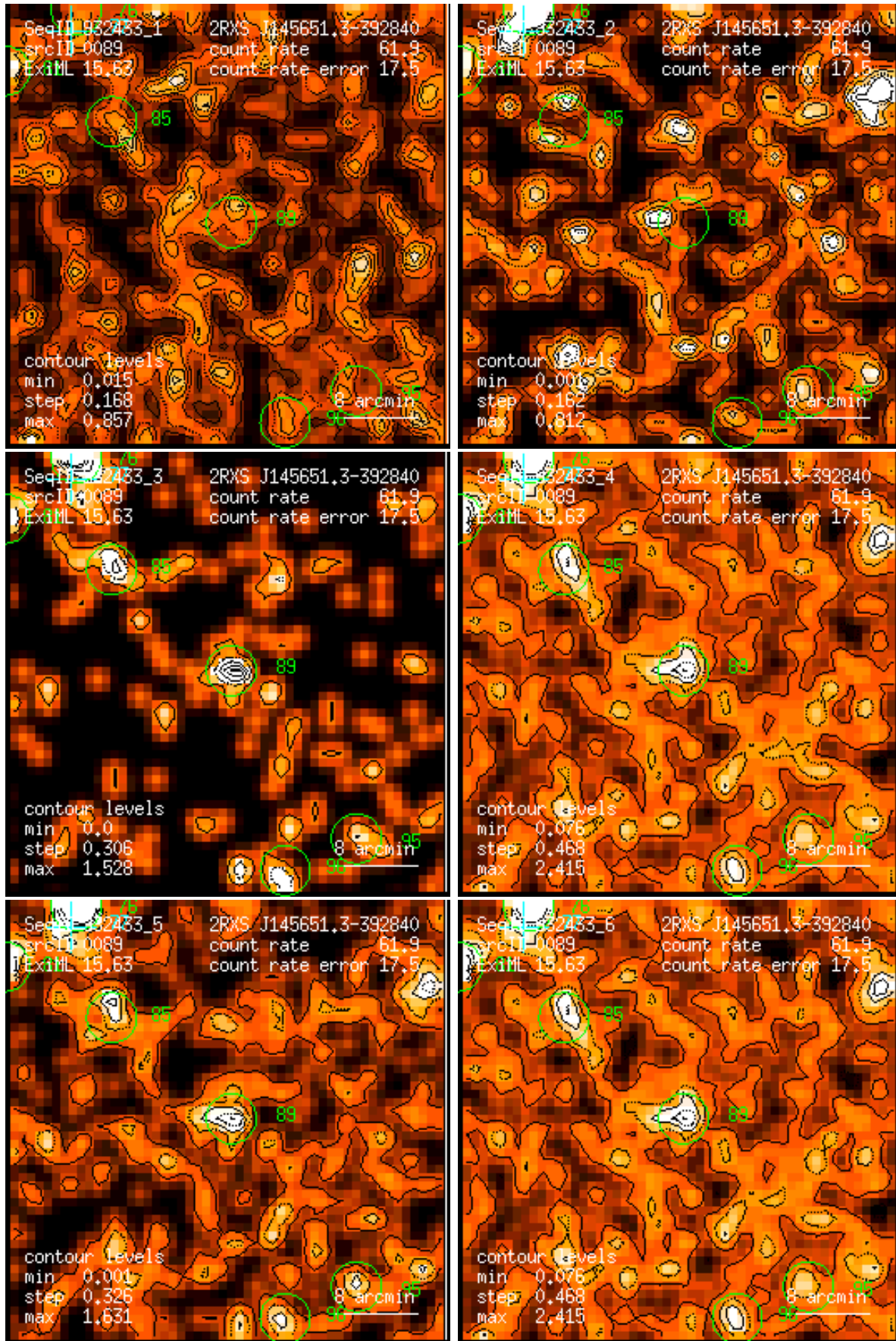
Figure 89: RASS 932433: detection 0089: band rate images, Gaussian filter: (1) PSPC channels 11 – 41, (2) 52 – 90, (3) 91 – 201, (4) 11 – 235, (5) 52 – 201, (6) 11 – 201. Broad band rates in counts/ks. Band rate contour levels in counts/ks/arcmin 2 .
