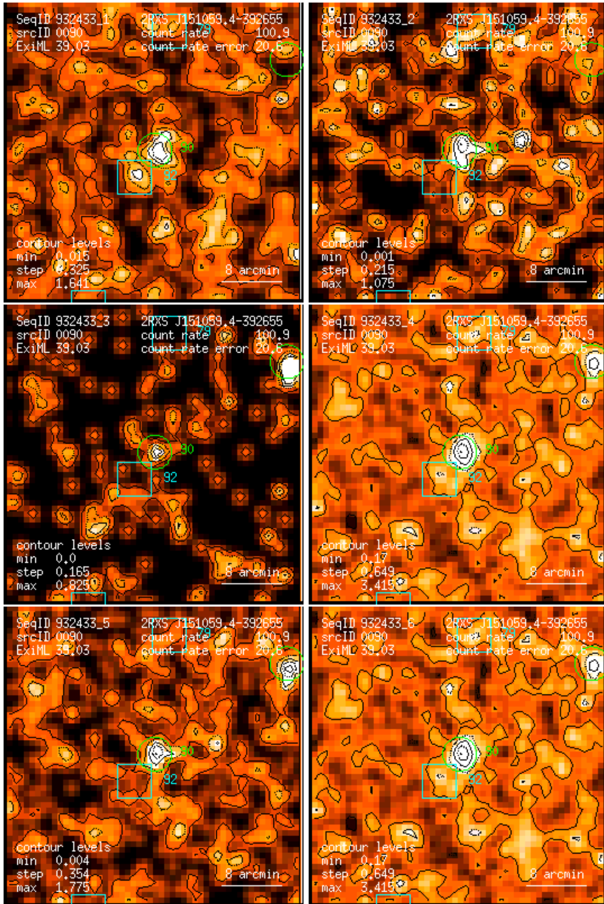
Figure 90: RASS 932433: detection 0090: band rate images, Gaussian filter: (1) PSPC channels 11 – 41, (2) 52 – 90, (3) 91 – 201, (4) 11 – 235, (5) 52 – 201, (6) 11 – 201. Broad band rates in counts/ks. Band rate contour levels in counts/ks/arcmin 2 .
