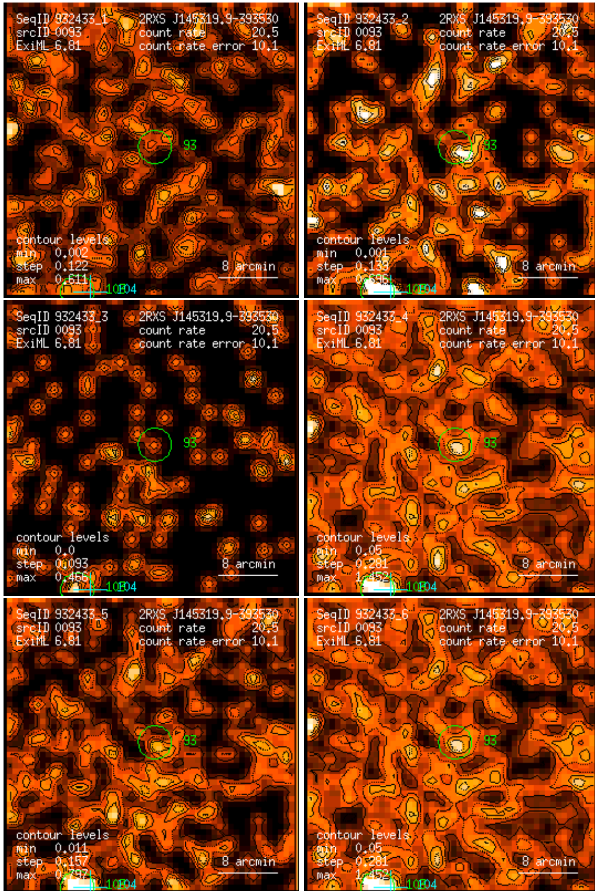
Figure 93: RASS 932433: detection 0093: band rate images, Gaussian filter: (1) PSPC channels 11 – 41, (2) 52 – 90, (3) 91 – 201, (4) 11 – 235, (5) 52 – 201, (6) 11 – 201. Broad band rates in counts/ks. Band rate contour levels in counts/ks/arcmin 2 .
