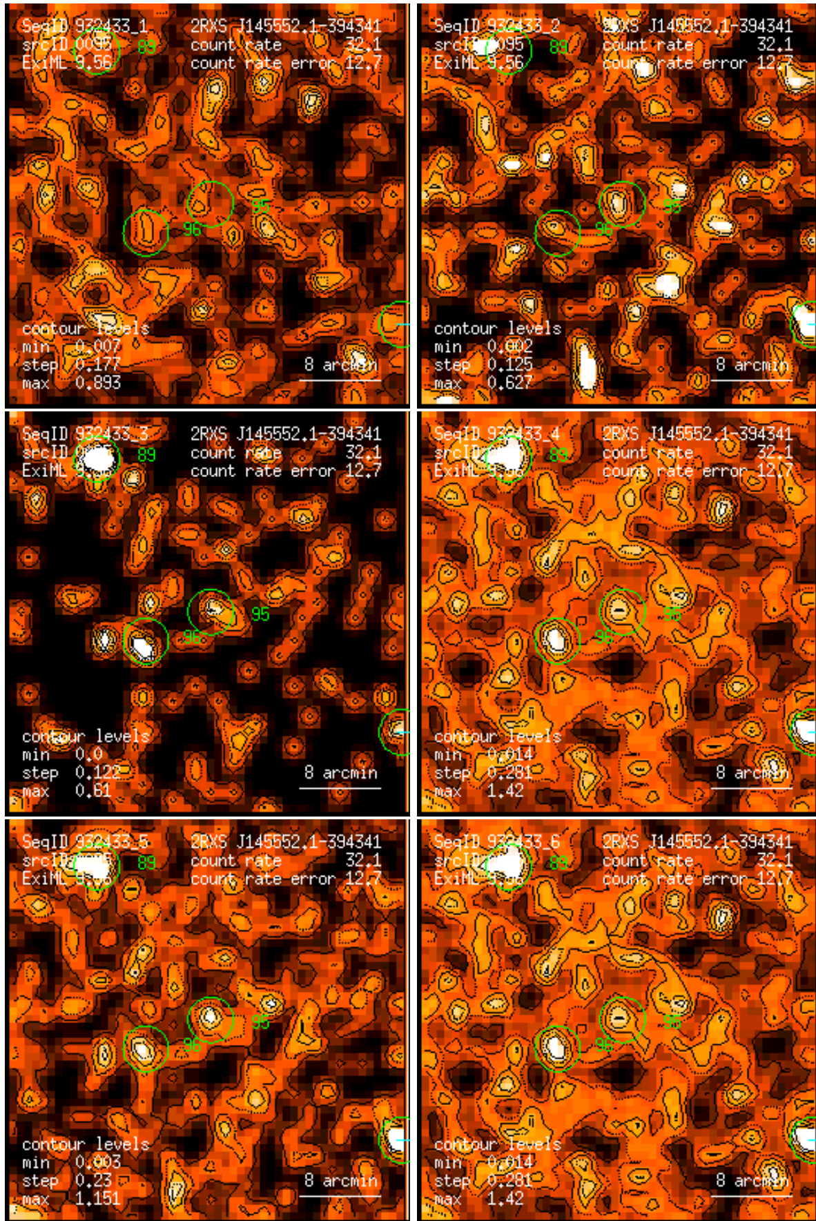
Figure 95: RASS 932433: detection 0095: band rate images, Gaussian filter: (1) PSPC channels 11 – 41, (2) 52 – 90, (3) 91 – 201, (4) 11 – 235, (5) 52 – 201, (6) 11 – 201. Broad band rates in counts/ks. Band rate contour levels in counts/ks/arcmin 2 .
