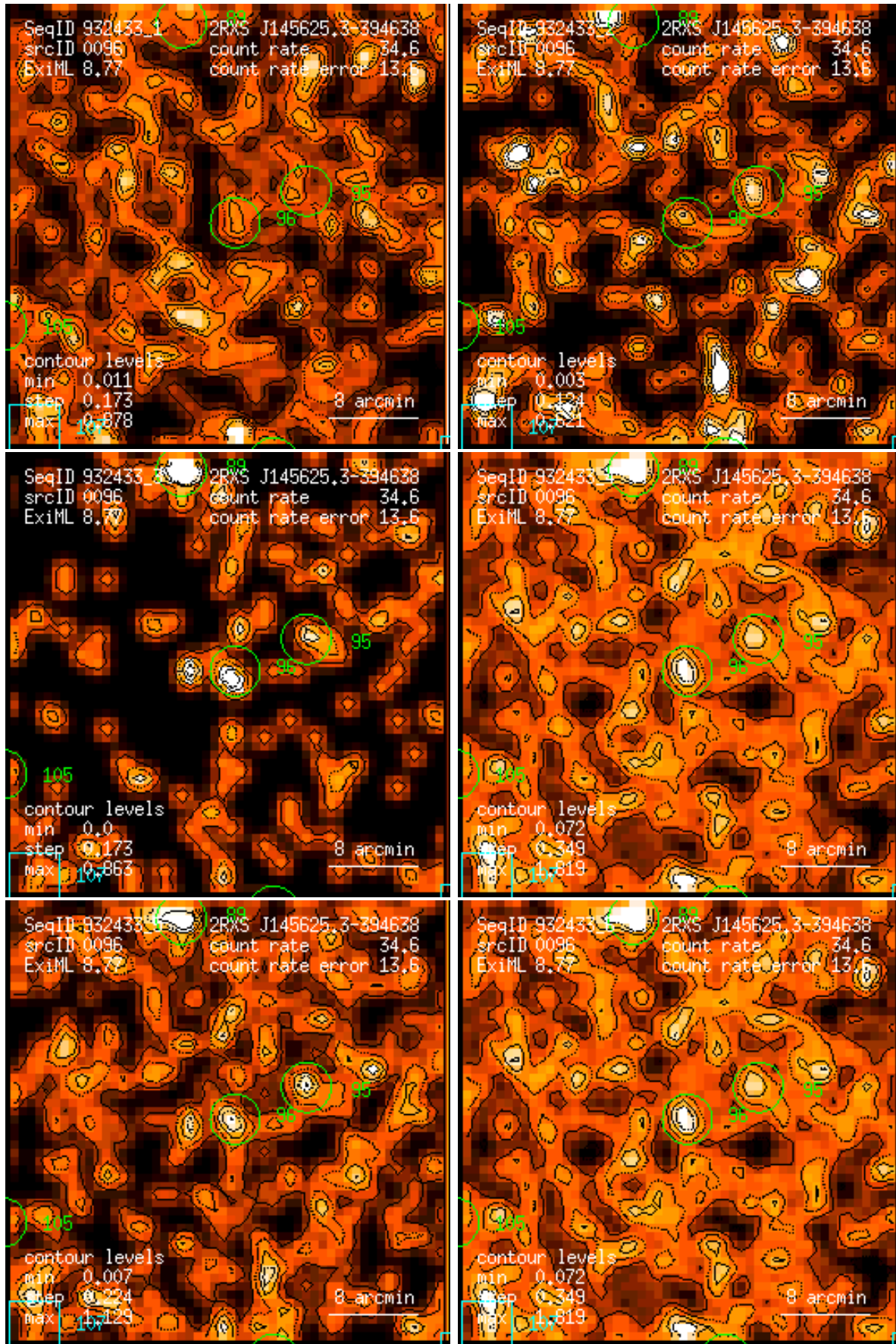
Figure 96: RASS 932433: detection 0096: band rate images, Gaussian filter: (1) PSPC channels 11 – 41, (2) 52 – 90, (3) 91 – 201, (4) 11 – 235, (5) 52 – 201, (6) 11 – 201. Broad band rates in counts/ks. Band rate contour levels in counts/ks/arcmin 2 .
