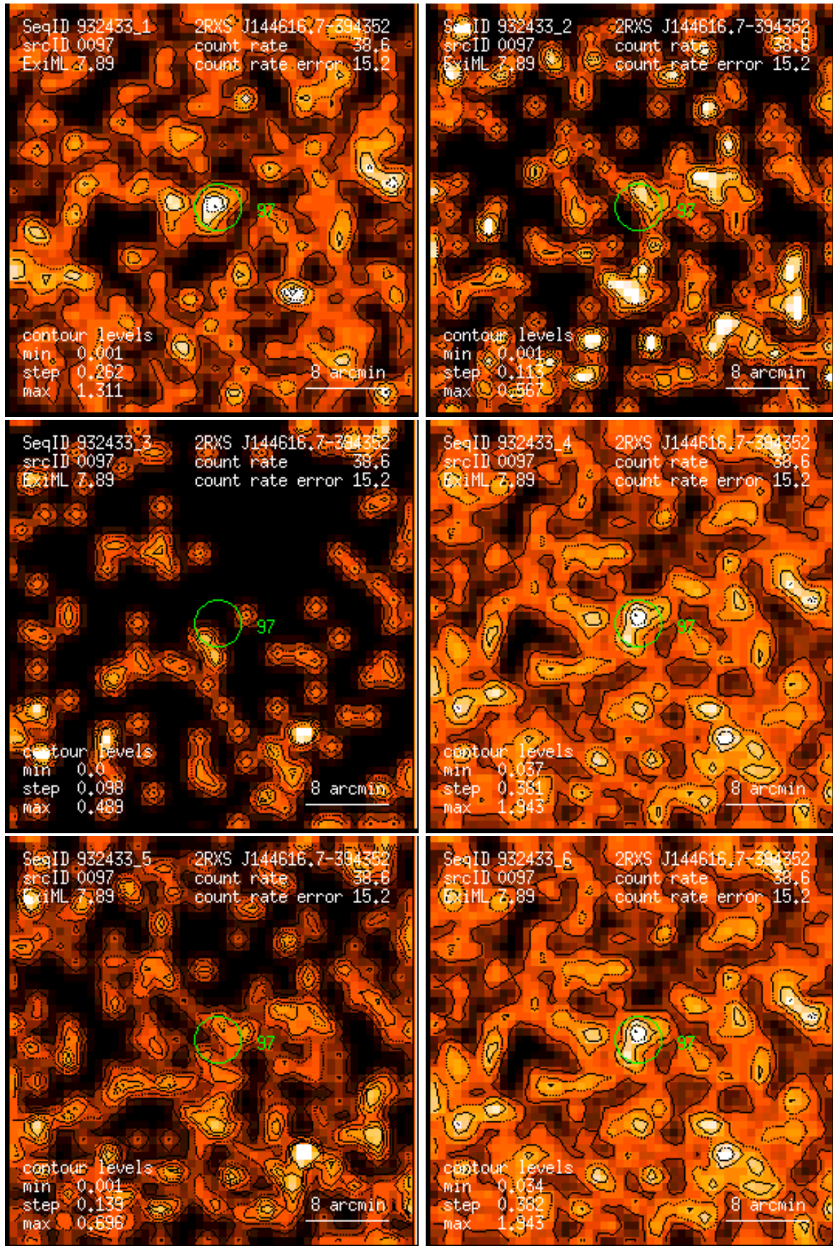
Figure 97: RASS 932433: detection 0097: band rate images, Gaussian filter: (1) PSPC channels 11 – 41, (2) 52 – 90, (3) 91 – 201, (4) 11 – 235, (5) 52 – 201, (6) 11 – 201. Broad band rates in counts/ks. Band rate contour levels in counts/ks/arcmin 2 .
