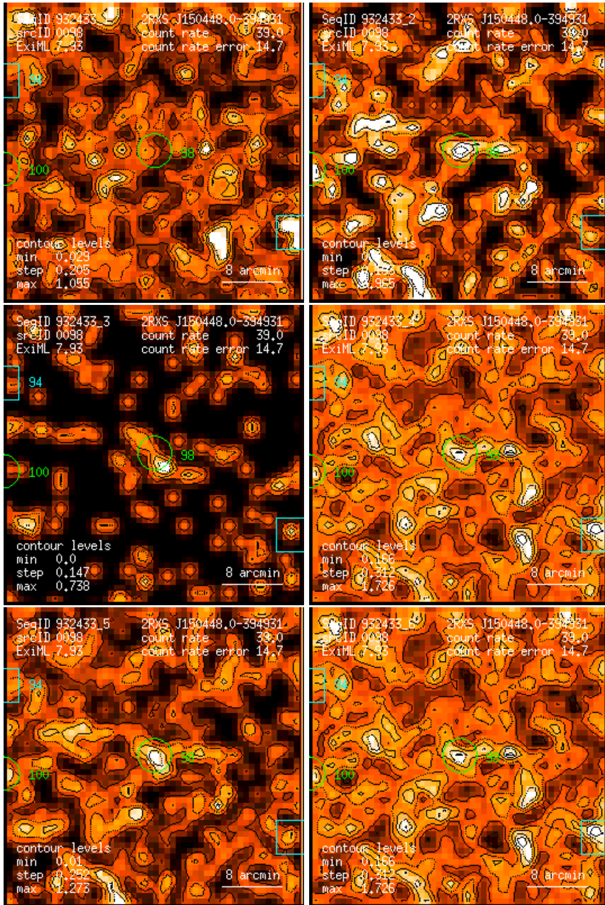
Figure 98: RASS 932433: detection 0098: band rate images, Gaussian filter: (1) PSPC channels 11 – 41, (2) 52 – 90, (3) 91 – 201, (4) 11 – 235, (5) 52 – 201, (6) 11 – 201. Broad band rates in counts/ks. Band rate contour levels in counts/ks/arcmin 2 .
